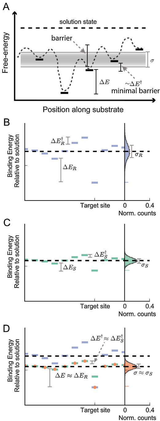
Fig. 2. Search-stability paradox.
