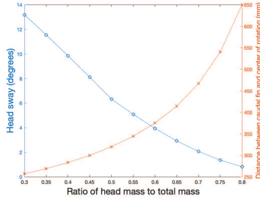
Fig. 6: Simulation results of the sway stability (circles) and maneuverability (crosses) versus the weight ratio of the head of the fish. The right axis indicates the distance between the caudal fin and the center of rotation, which is inversely related to the maneuverability.
