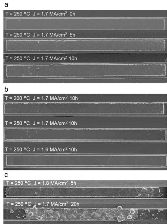
FIG. 4. SEM images of Blech structure lines after different EM conditions. (a) 60 \mu\text{m} stripes under J_{\text{EM}} = 1.7 \text{ MA cm}^{-2} at 250^\circ\text{C} from 0 to 10 h; (b) 60 \mu\text{m} stripes under J_{\text{EM}} = 1.7 \text{ MA cm}^{-2} and J_{\text{EM}} = 1.6 \text{ MA cm}^{-2} at 200 and 250^\circ\text{C} at 10 h; and (c) 60 \mu\text{m} stripes under higher current density J_{\text{EM}} = 1.8 \text{ MA cm}^{-2} at 5 h and extended EM duration J_{\text{EM}} = 1.7 \text{ MA cm}^{-2} at 20 h.
