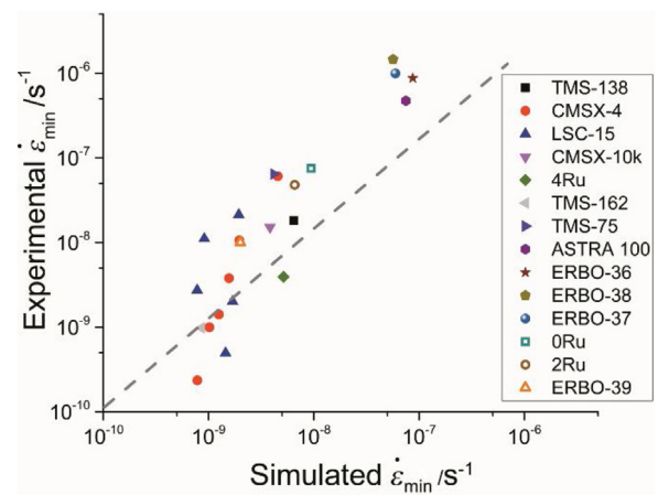
Fig. 6. Simulated minimum creep rate of existing Ni commercial grades compared with the experimental results obtained from the literature [65,77,91–94].
