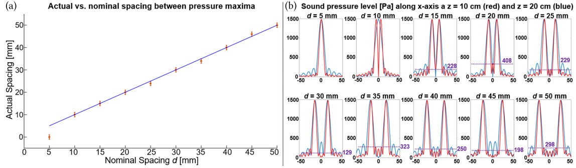
Fig. 9. Simulation of focal point pairs with identical spacing to those used in the human participant study, on the same array but at a height of z = 10 cm above the array. (a) The relationship between actual and nominal spacing. (b) Plots of the acoustic pressure along the x axis in red, overlaid on the plots from Figure 7 (at z = 20 cm) in blue.
