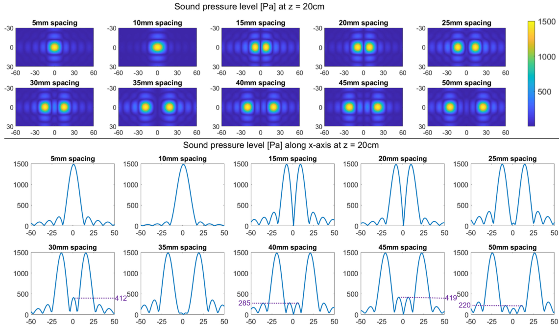
Fig. 7. (Top) Heat maps showing the sound pressure level in the plane at z = 20 cm above the array (in Pa). (Bottom) Sound pressure plots along the y = 0 axis in the same plane (in Pa). Notable pressure lobes occurring between the peaks around the focal points are annotated with their peak pressure value (in Pa) in purple.
