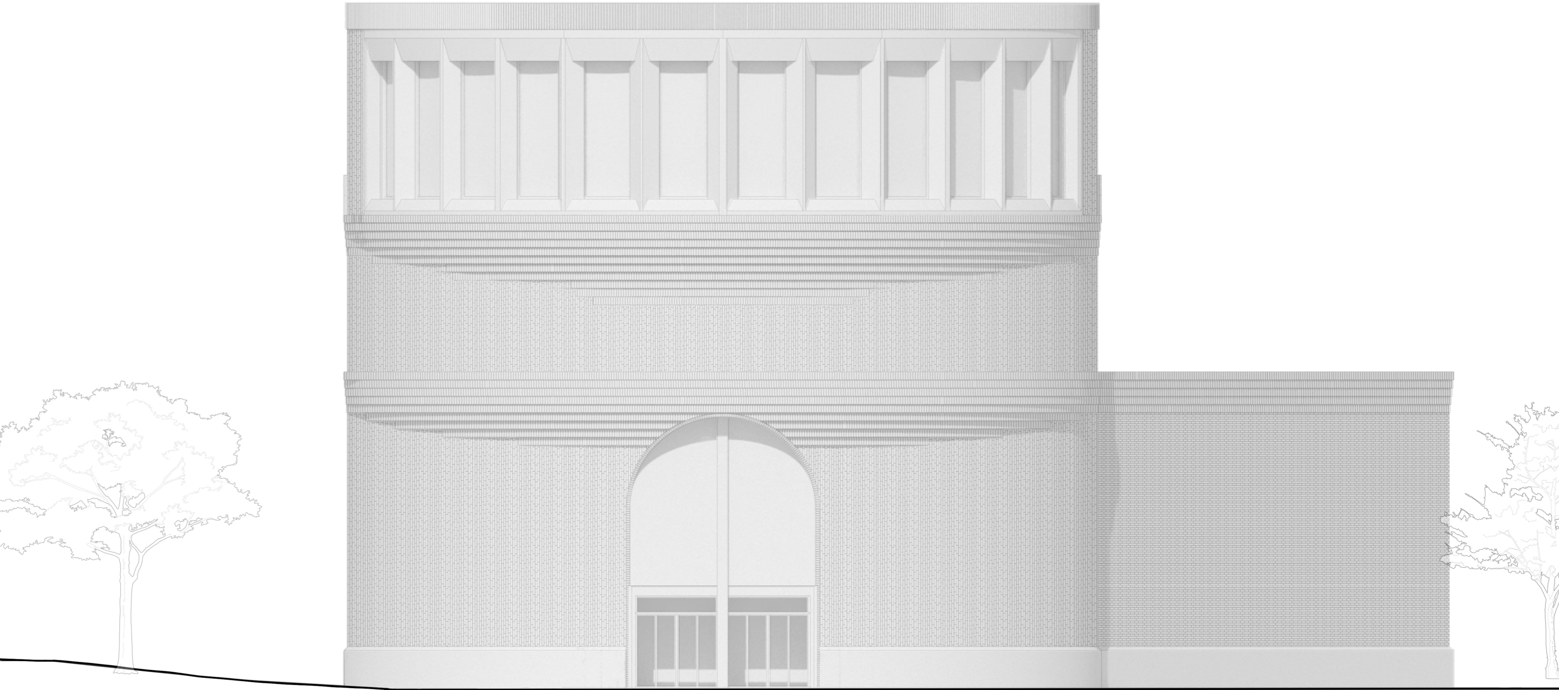
North Elevation 1:100
