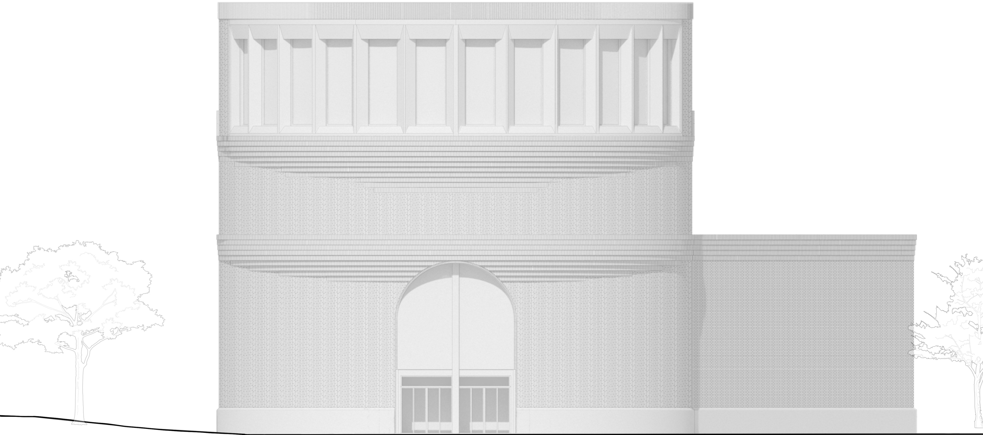
North Elevation 1:100
