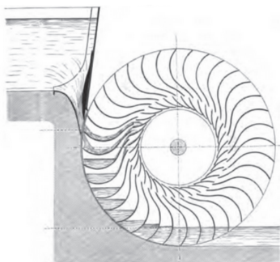
Figure 3-11: Zuppinger wheel
