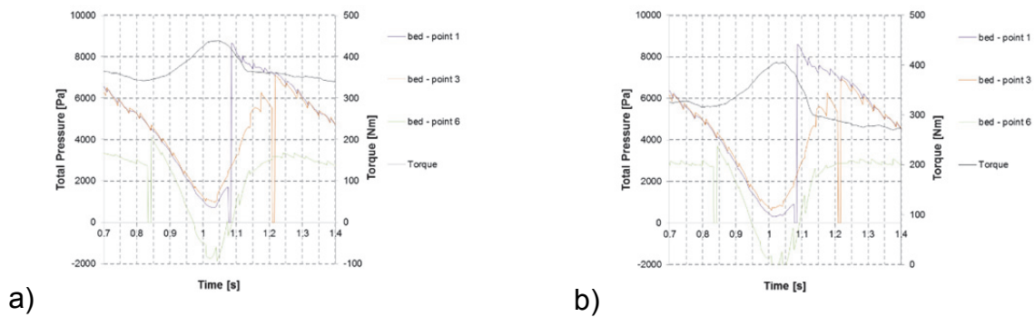
Figure 6-89: Total pressure below wheel at channel bed, (a) parallel walls, (b) diffuser
