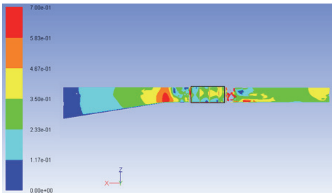
Figure 6-18: Surface velocity contours in m/s (discharge = 0.18 \text{ m}^3/\text{s} , \Delta h = 0.619 \text{ m} )
