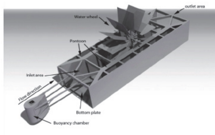
Figure 7-4: CAD model of the free stream energy converter
