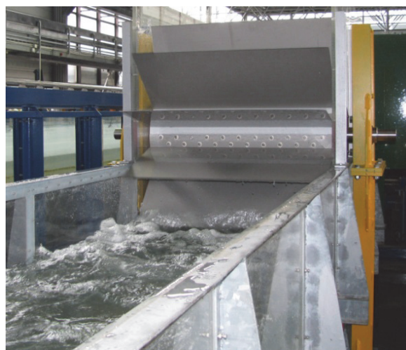
Figure 2-12: Laboratory model (view from downstream)
