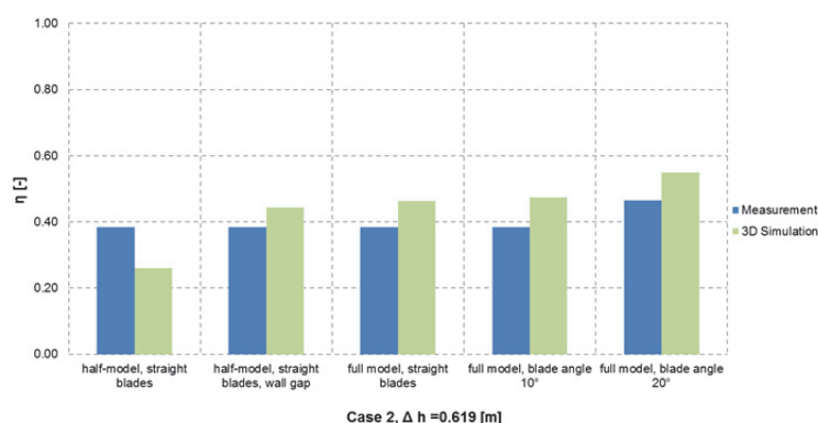
Figure 6-65: Addition of features in the simulation models
