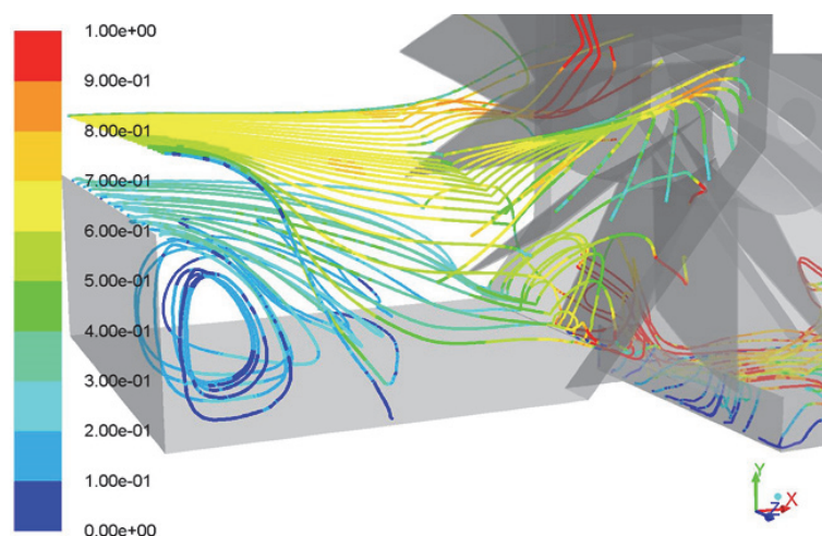
Figure 6-71: Velocity pathlines
