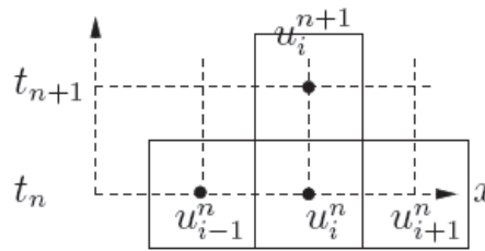
Figure 4-1: Upwind discretisation
