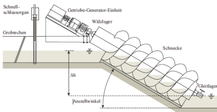
Figure 3-13: Hydrodynamic screw
