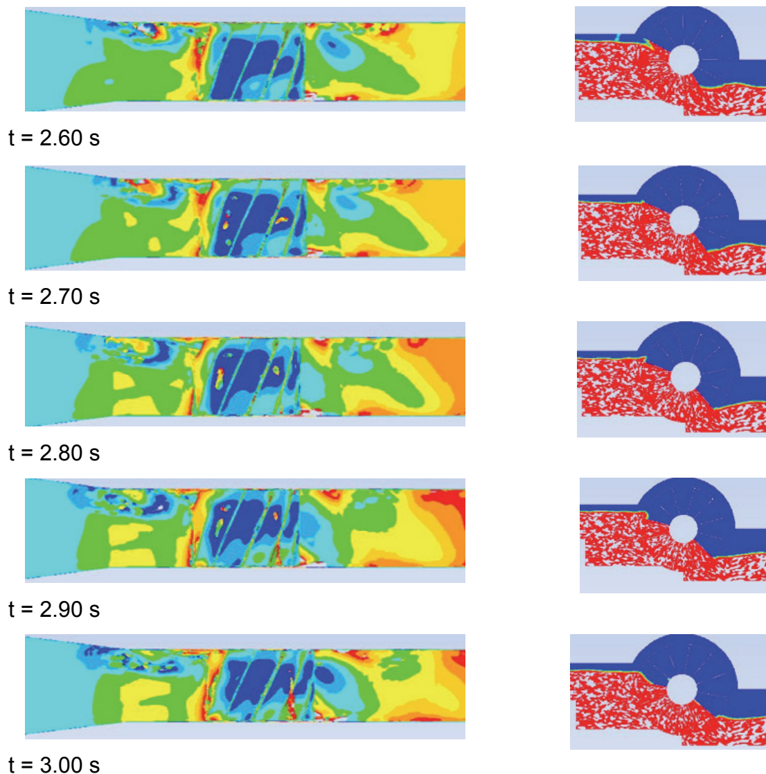
Figure 6-54: Free surface velocities, air-water phases ( t = 2.6 s to 3.0 s)
