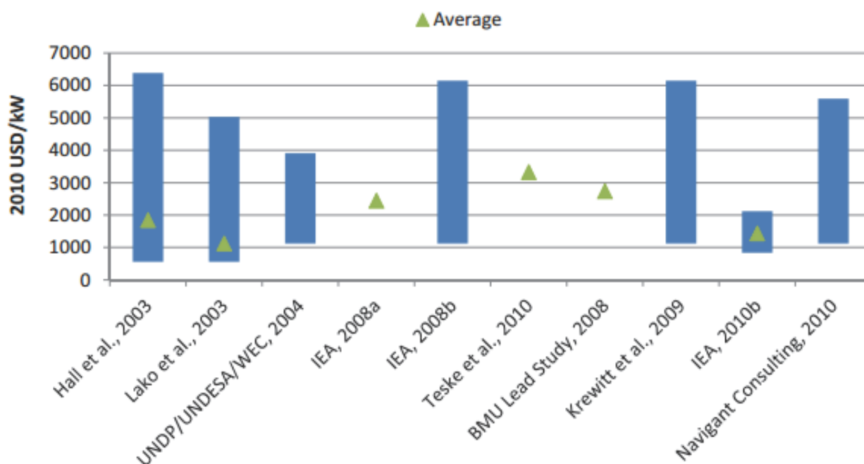
Figure 2-5: Range of installed costs of hydropower from different studies
