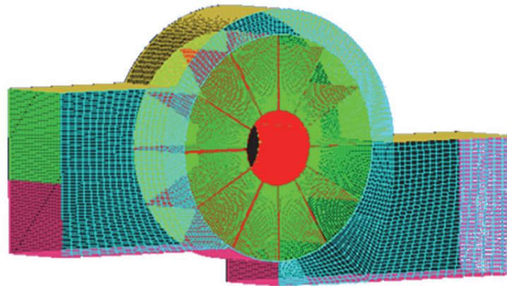
Figure 6-4: Mesh with straight blades
