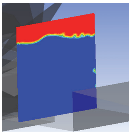
Figure 6-61: Water level, upstream
