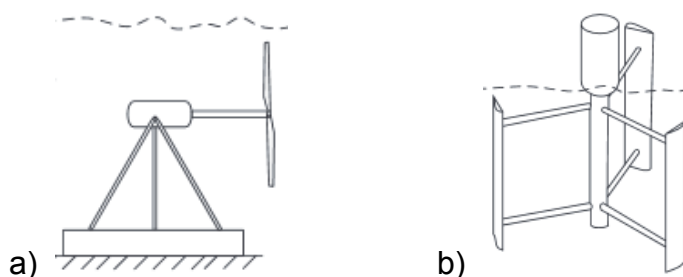
Figure 3-16: Free-flow turbines: a) axial turbine, b) cross flow Darrieus turbine
