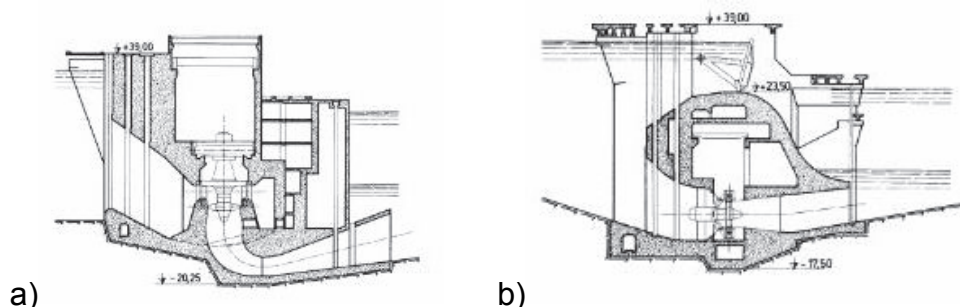
Figure 3-2: Kaplan (a) and Straflo (b) turbines
