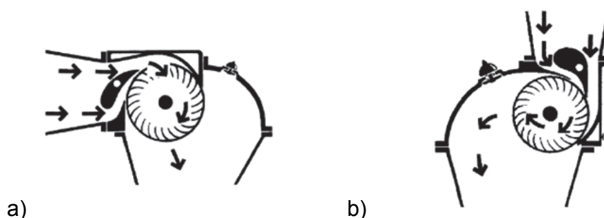
Figure 3-6: Cross flow turbine with (a) horizontal inlet and (b) vertical inlet
