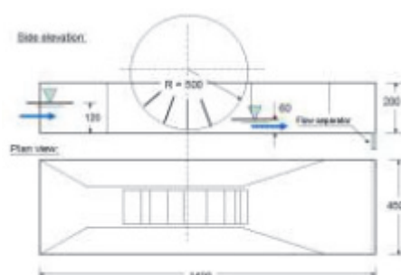
Figure 3-22: Free stream energy converter
