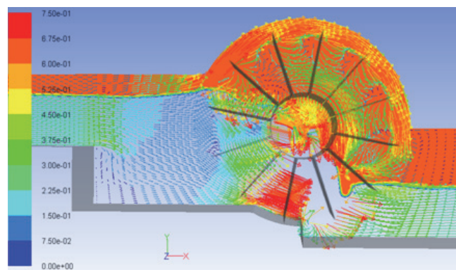
Figure 6-27: Flow velocities at left wall (discharge = 0.18 m 3 /s, \Delta h = 0.619 m) with symmetry plane
