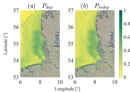
Fig. E.4. The spatial probabilities with (a) accounting for dependence ( P_{dep} ) and (b) without ( P_{ind} ), describing the suitability of blue mussel Mytilus edulis for the optimal growth conditions.
