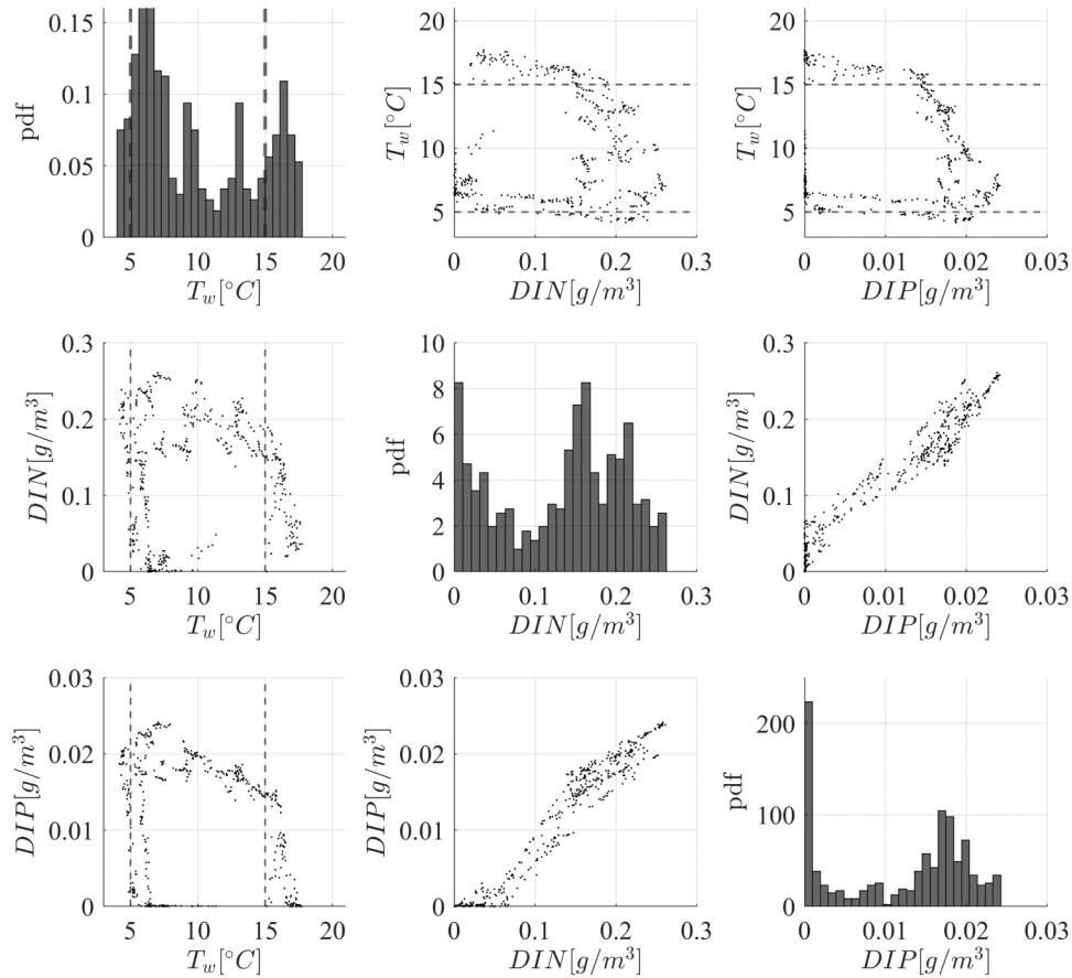
Fig. F.1. Overview of sampled data for sugar kelp at the location of the FINO3 research platform together with the optimal limits from Table 1, while on the diagonal the empirical probabilistic distribution functions (pdf's) are shown.
