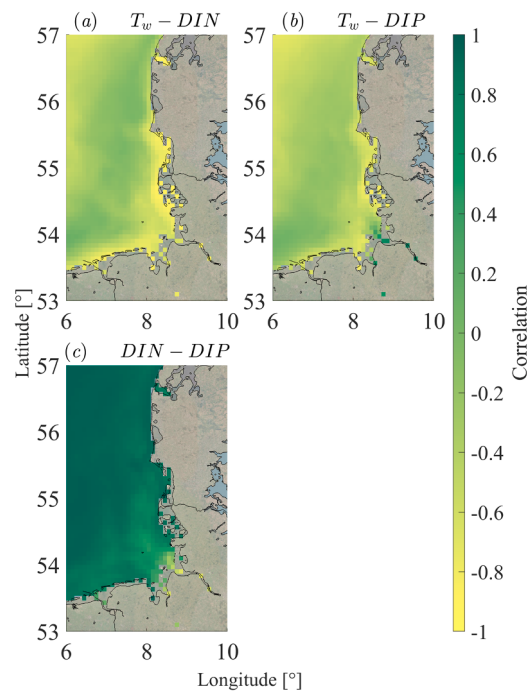
Fig. F.3. Correlations between the selected three variable pairs for the sugar kelp: (a) T_w and DIN , (b) T_w and DIP and (c) DIN and DIP .
