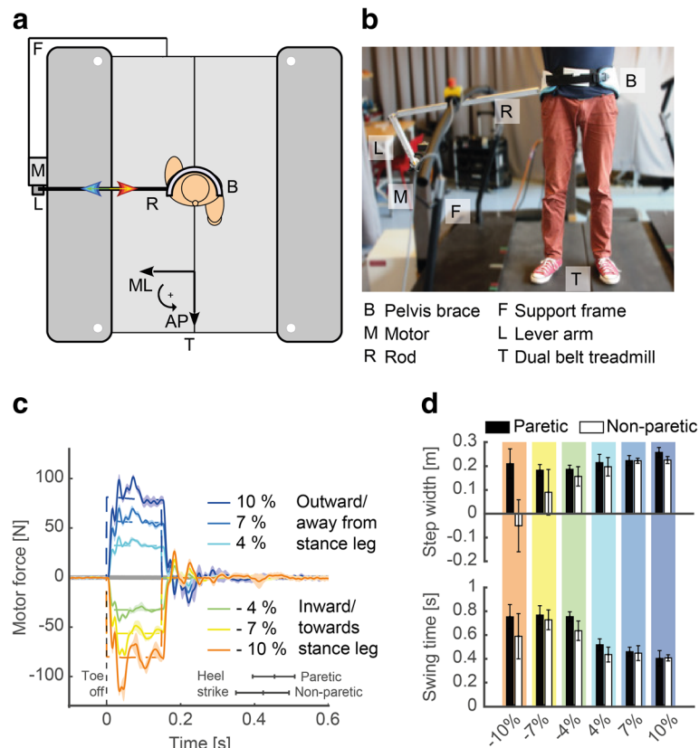
Fig. 2 To systematically assess how patients maintain their balance when being perturbed during walking, the University of Twente has developed a pelvic perturbation device ( a and b ) [36]. This device consists of an admittance-controlled motor (Moog, Nieuw Vennep, the Netherlands) connected via a lever arm and a rod to a pelvic brace worn by the subject. The device allows providing perturbations in different directions, with different magnitudes and different durations at precisely timed instances of the gait cycle while walking on a treadmill ( c , mediolateral perturbations timed at toe off with magnitudes expressed as % of body weight). In collaboration with Roessingh Research & Development, the device was used to assess the foot placement strategies of ambulatory stroke survivors when being perturbed away or towards the stance leg at the start of swing of the paretic or non-paretic legs. Responses of the step directly following the perturbation in a single stroke survivor are indicated in ( d ). Whereas the stroke survivor made a cross step, as evidenced by the negative step width, with his non-paretic leg when being forcefully perturbed towards the paretic leg, he did not make a cross step with his paretic leg. When being perturbed away from the stance leg, both the paretic and non-paretic side only slightly adjusted the step width but the foot was placed faster on the ground, as evidenced by the decreased swing time, to counteract the perturbation
