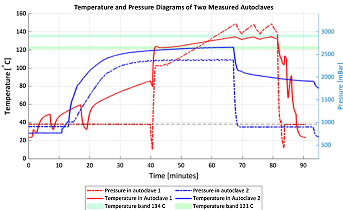
Fig. 2 Temperature and pressure diagrams of the two measured autoclaves. The graphs show the readout of pressure and temperature sensors placed into the autoclave chamber during one cycle
