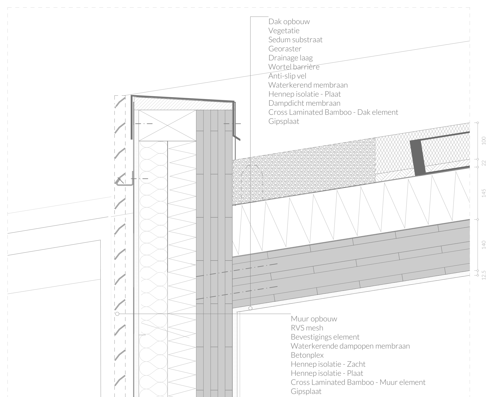
Detail D: Dakrand 1:5
