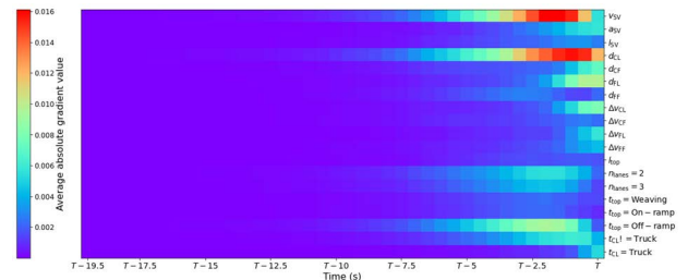
FIGURE 9. Heat map showing the dynamic gap selection process of trucks.
