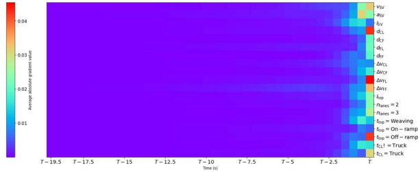
FIGURE 5. Heat map showing the dynamic gap selection process of passenger cars.
