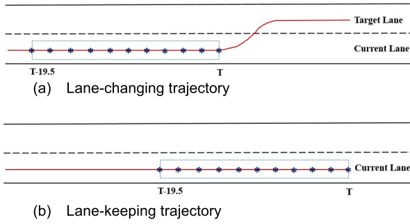
FIGURE 3. Figure showing span and data sampling for (a) lane-changing and (b) lane-keeping trajectories of drivers (Note: * denotes a data sampling instant at a resolution of 0.5 s.)
