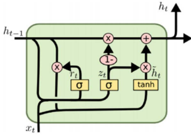
FIGURE 1. Architecture of a GRU cell (adapted from (Cho et al. [20])).
