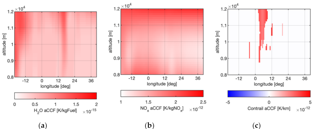
Figure 2. Algorithmic climate change functions for H 2 O (a), NO x (b), and contrails (c) on 18 December 2015, 6.00 p.m. UTC as function of longitude and altitude at 48° N.
