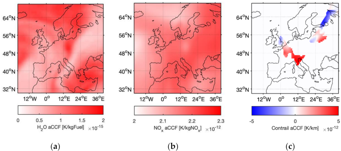
Figure 1. Algorithmic climate change functions for H 2 O (a), NO x (b), and contrails (c) on 18 December 2015, 6.00 p.m. UTC as function of latitude and longitude on flight level 390.
