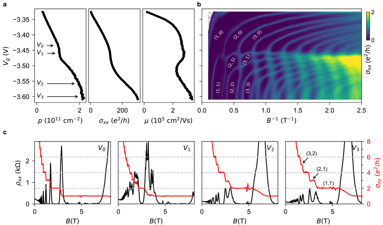
Figure 2. a) From left to right: gate voltage ( V_g ) dependence of the hole bilayer Hall density p , conductivity \sigma_{xx} at zero magnetic field, and mobility \mu . The bilayer behavior at V_g = V_0, V_1, V_2 , and V_3 is further described in the main text. b) Color map of the conductivity \sigma_{xx} as a function of V_g (same range as in (a)) and the inverse magnetic field B^{-1} . Dark regions correspond to filled Landau levels with vanishing \sigma_{xx} and correspondingly quantized \sigma_{xy} . In brackets the filling factor ( \nu_{\text{sbb1}}, \nu_{\text{sbb2}} ) for the first and second subbands where \nu = 0 indicates an empty subband. c) From left to right: \rho_{xx} (black) and \sigma_{xy} (red) as a function of magnetic field B at V_g = V_0, V_1, V_2 , and V_3 . These line cuts are obtained from the magnetotransport measurement in (b). \sigma_{xy} shows plateaus at integer values of the total filling factor ( \nu_{\text{sbb1}} + \nu_{\text{sbb2}} ).
