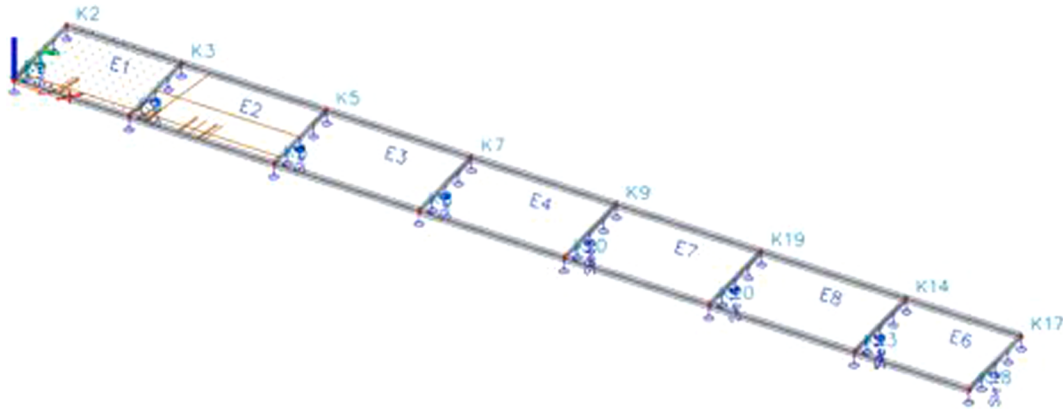
Fig. 13. Overview of linear finite element model.
