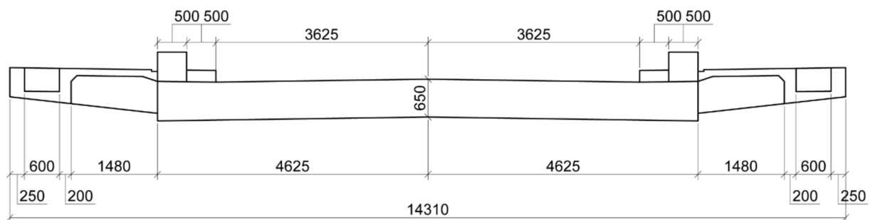
Fig. 8. Cross-sectional view of the Nieuwklap Bridge. Units: mm.
