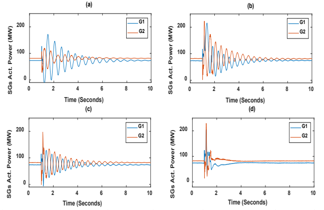
Figure 7. Active Power from SGs due to a Fault at Bus 8- 6 cycles: a) only SGs connected, b) Basic LVRT controller applied in WGs, c) VDAPI LVRT controller applied in WGs, d) SDC LVRT controller applied in WGs
