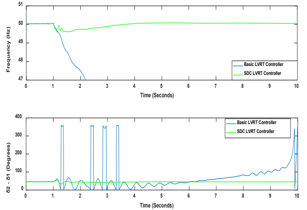
Figure 9. Frequency & Rotor angle responses with 75% WG share
