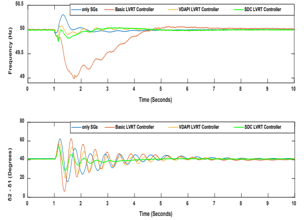
Figure 8. 52% WG share Frequency & Rotor angle responses
