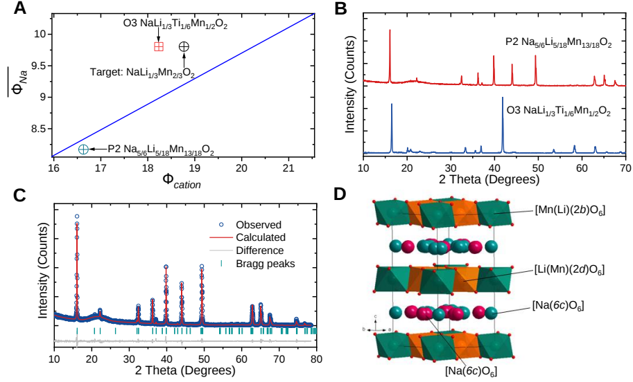
Fig. 3. Designing P2-type oxide. (A) Analysis of cationic potential of Na-Li-Mn-O oxides (see Table S13 and S14 for details). (B) XRD patterns of NaLi_{1/3}Ti_{1/6}Mn_{1/2}O_2 and Na_{5/6}Li_{5/18}Mn_{13/18}O_2 oxides. (C) Rietveld refinement of XRD pattern of Na_{5/6}Li_{5/18}Mn_{13/18}O_2 (see Table S15-17 for details). (D) Schematic illustration of the corresponding structure with the Li/Mn ordering in the [Li_{5/18}Mn_{13/18}]O_2 slabs.
