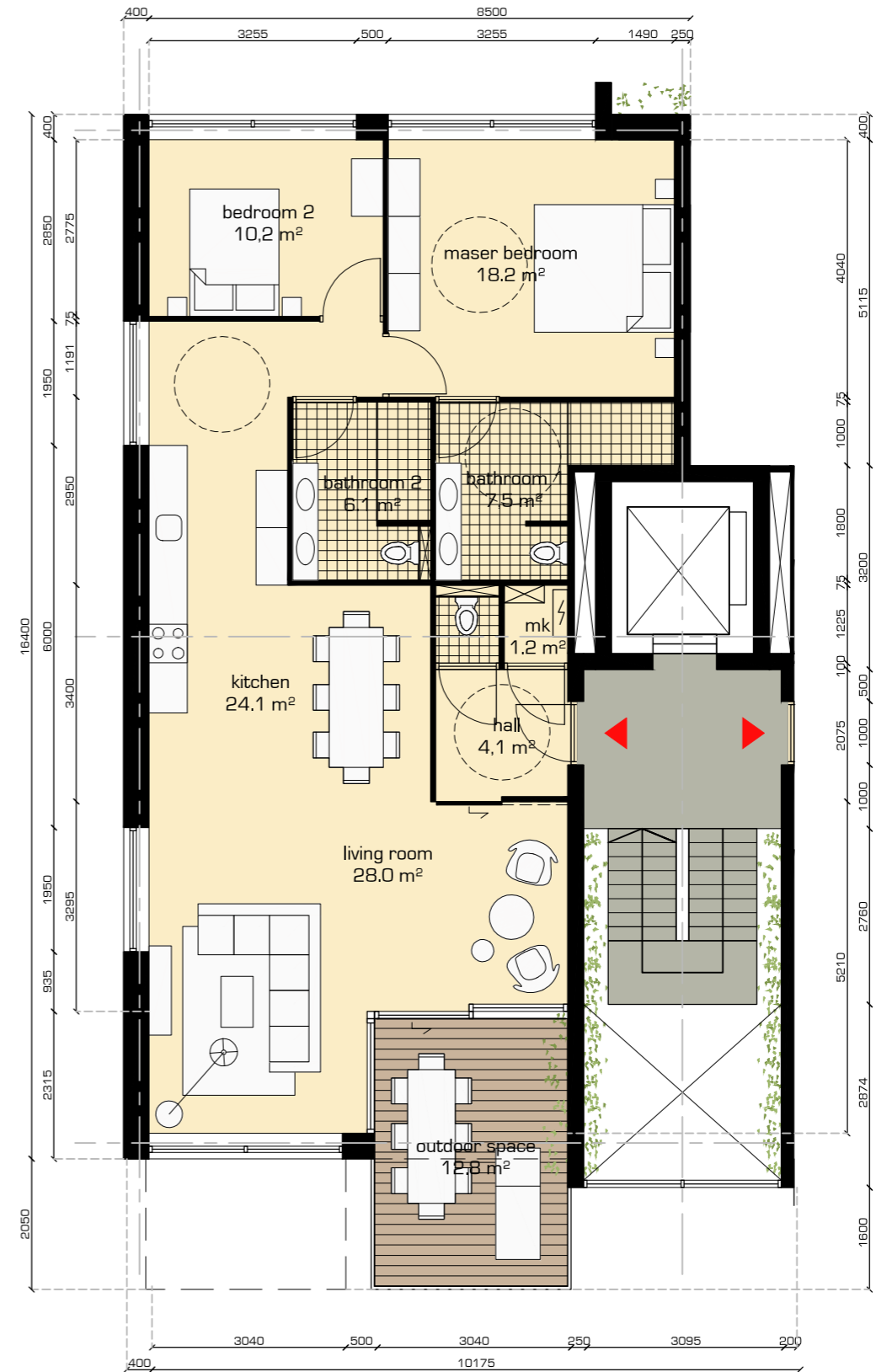
type B floorplan 105 m 2 (1:100)
