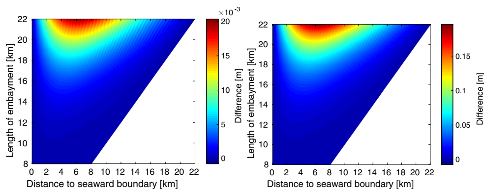
Fig. 4 The influence of the bottom friction parameter for a diverging embayment. The colourplots show the difference between the bed profiles when friction is included and not included, left: ( \text{sol}_{c_d=0.001} - \text{sol}_{c_d=0} ) and right: ( \text{sol}_{c_d=0.003} - \text{sol}_{c_d=0} ). The embayment length is varied between L = 8 km and L = 22 km (vertical axis) and the distance to the seaward boundary on the horizontal axis. The colour indicates the influence of bottom friction: the blue colours indicate that
