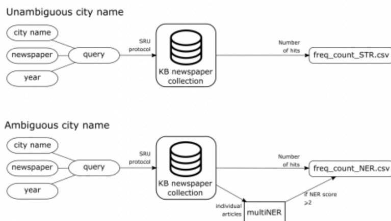
Figure 5: Data collection algorithms
