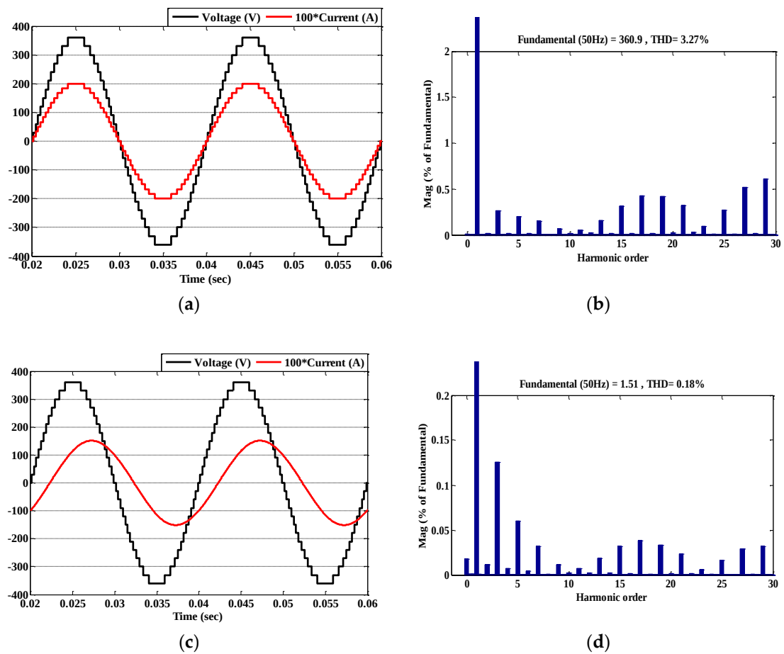
Figure 8. Simulation results of a 25-level inverter of the proposed topology: (a) output waveforms of a resistive load ( R = 180 \Omega ); (b) fast Fourier transform (FFT) analysis on the output voltage; (c) output waveforms of a resistive-inductive load ( R = 180 \Omega , L = 500 \text{ mH} ); (d) FFT analysis on the load current.
