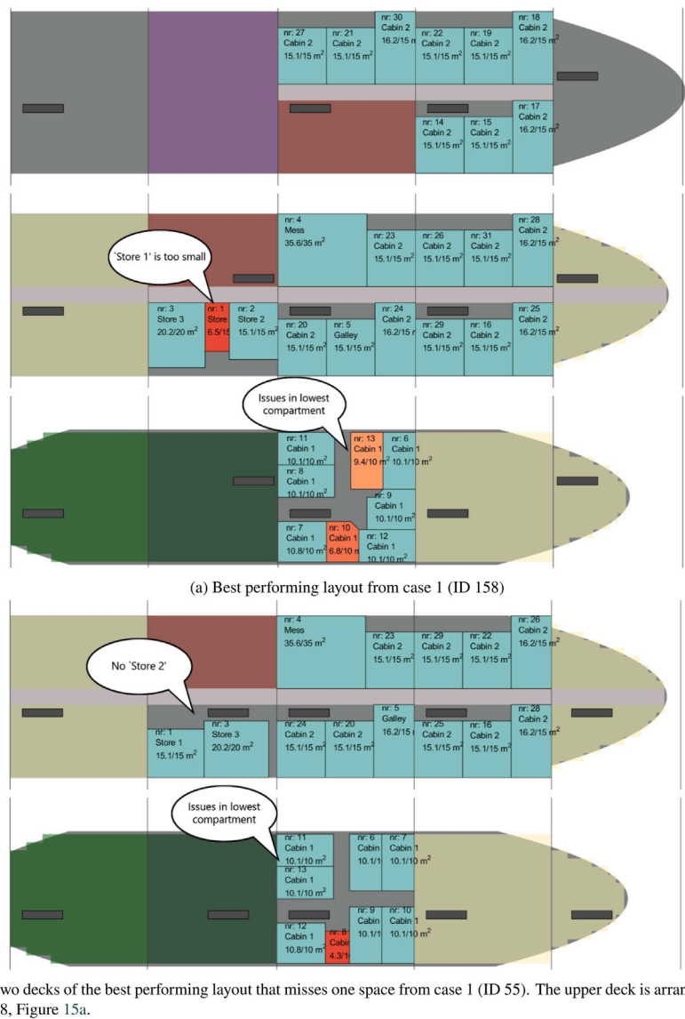
Fig. 15. Two selected layouts from case 1.
