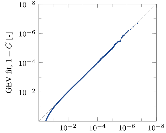
Figure 6. Q-Q plot, showing how well the empirical tail behavior matches a generalized extreme value distribution ( \mu = 78.2 \text{ MN} \times \text{m} ; \sigma = 2.05 \text{ MN} \times \text{m} ; \xi = 0.026 ).
