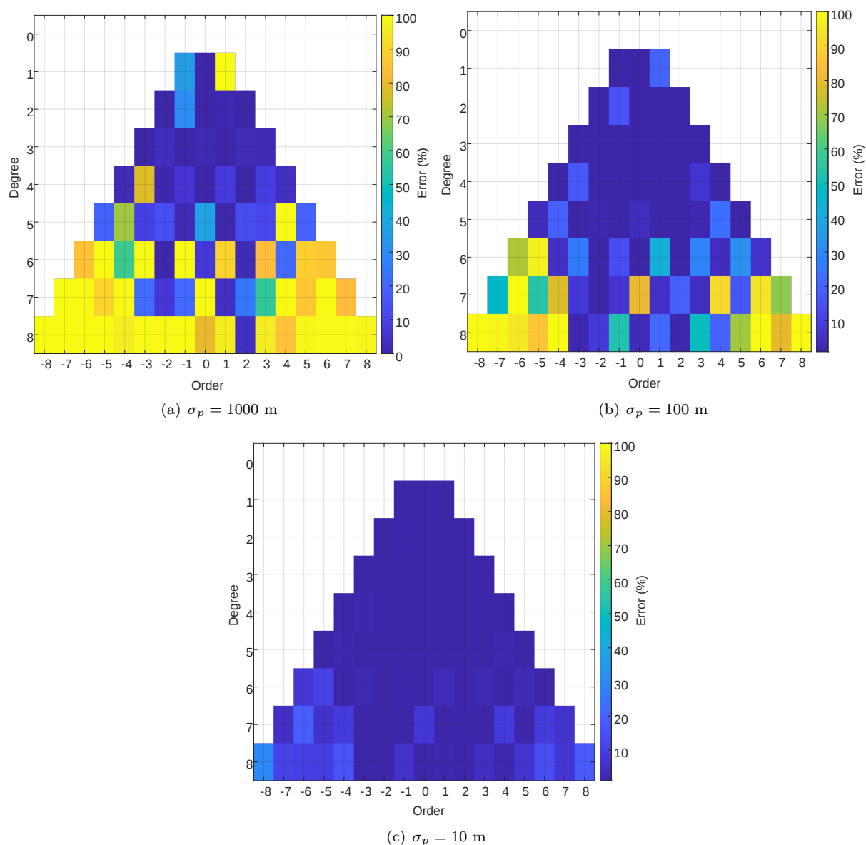
Figure 6. Coefficient-estimation errors as a function of position-measurement noise, \sigma_p . Orbital radius 45 km.
