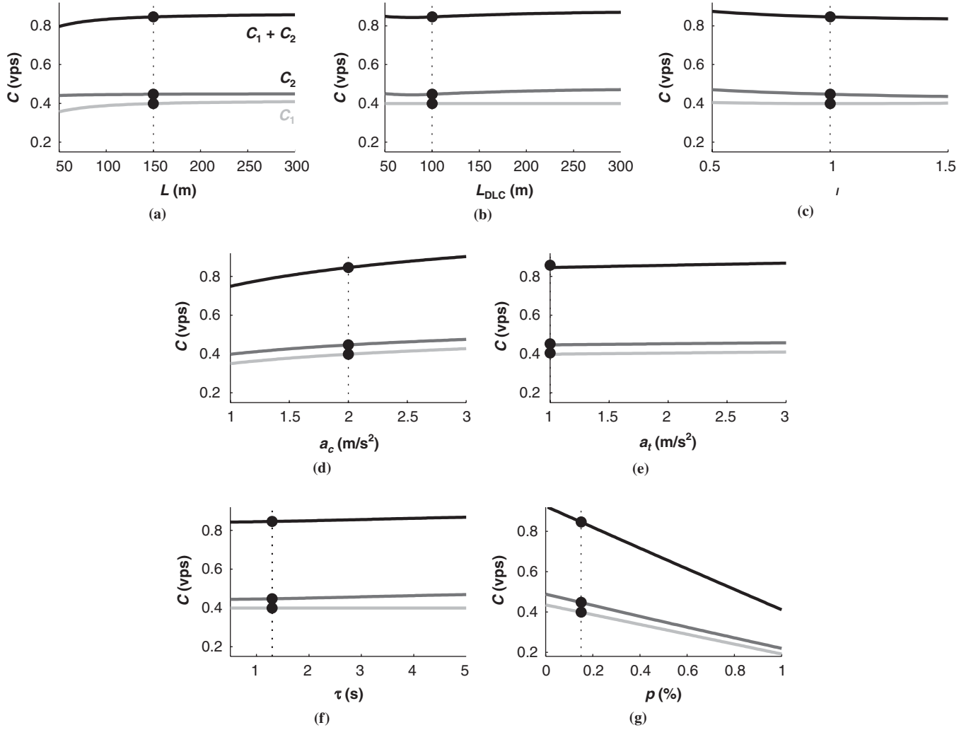
FIGURE 3 Sensitivity analysis by parameter: (a) length of the on-ramp ( L ), (b) length of the discretionary lane-changing area ( L_{DLC} ), (c) local merge ratio ( \alpha_l ), (d) car acceleration ( a_c ), (e) truck acceleration ( a_t ), (f) time to complete a lane-changing maneuver ( \tau ), and (g) fraction of trucks ( p ).
