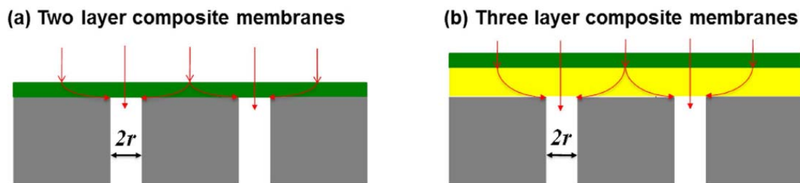
Figure 1.7. Schematic of thin film composite membranes: (a) with no PDMS gutter layer and (b) with PDMS gutter layer. Reproduced from ref [62]
