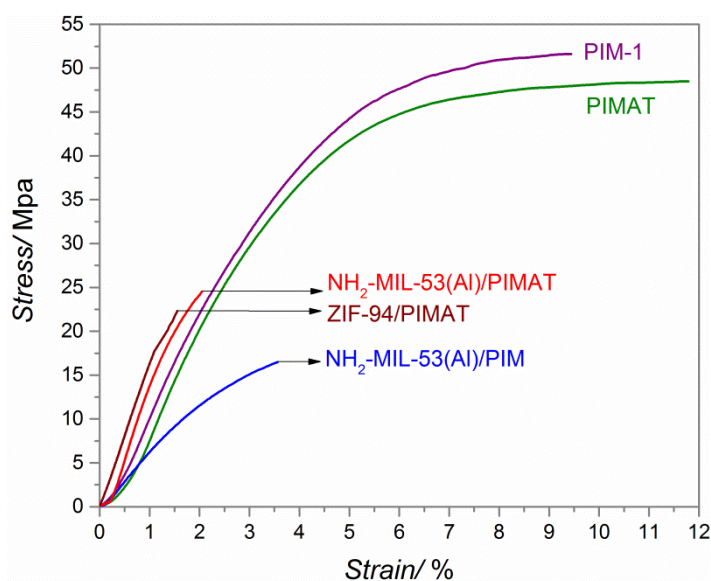
Figure 4.9. Stress versus strain curve of PIM-1, PIMAT, \text{NH}_2\text{-MIL-53(AI)/PIMAT} , ZIF-94/PIMAT and \text{NH}_2\text{-MIL-53(AI)/PIM-1} membranes.
