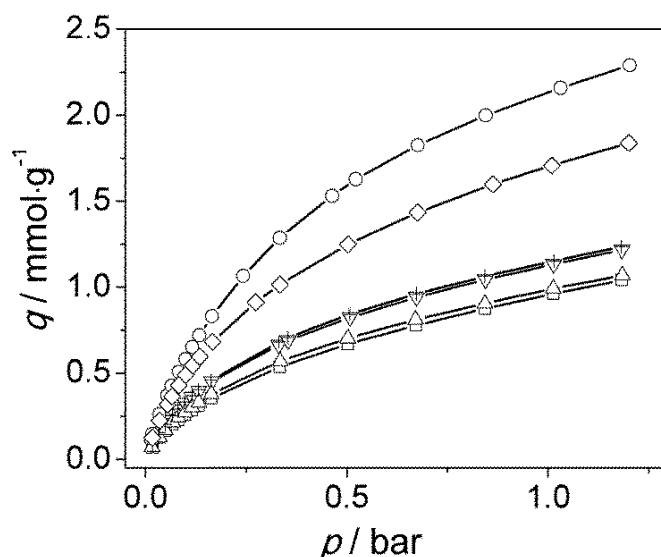
Figure 3.10 CO 2 adsorption isotherms acquired at 273 K, \diamond bare 6FDA-DAM, \circ 8 wt% NP-NH 2 -MIL-53(Al)@6FDA-DAM, \square bare Matrimid® and 8 wt% NH 2 -MIL-53(Al)@ Matrimid® with +NP, \Delta NR and MN.
