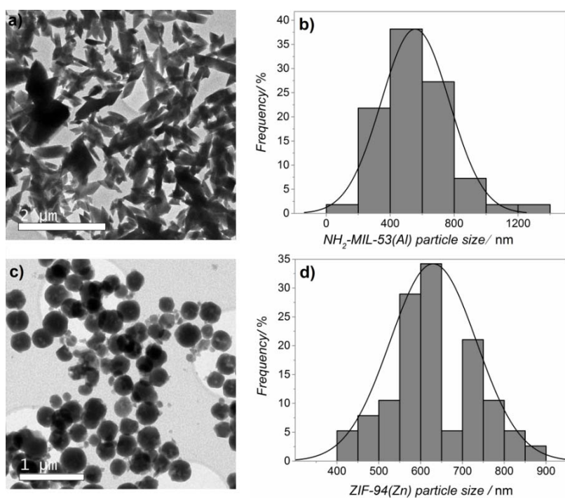
Figure 4.3 TEM images and particle size distribution of \text{NH}_2\text{-MIL-53(Al)} (a, b) and \text{ZIF-94(Zn)} (c, d).
