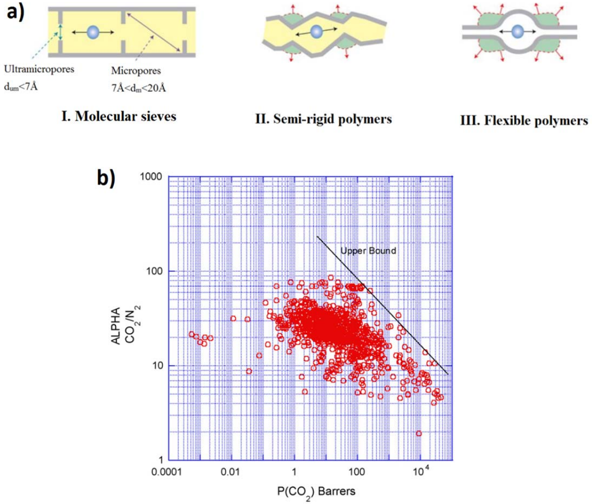
Figure 1.3. Molecular sieves with a rigid ultramicropore and micropore morphology (type I), Semi-rigid polymers with a distribution of connected pores created by segmental packing (type II), Flexible polymers with a transient gap distribution created by segmental packing and motion (type III) (a). Reproduced from ref [9], Upper bound correlation for CO_2/N_2 separation (b). Reproduced from ref [8b]
