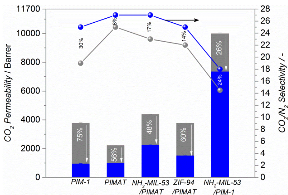
Figure 4.10 CO 2 and N 2 gas separation performance of the fresh (grey symbols and bars) and 90 days aged membranes (blue symbols and bars) (CO 2 and N 2 (15/85 vol.%) mixture was used as feed at 298 K and 2 bar absolute).
