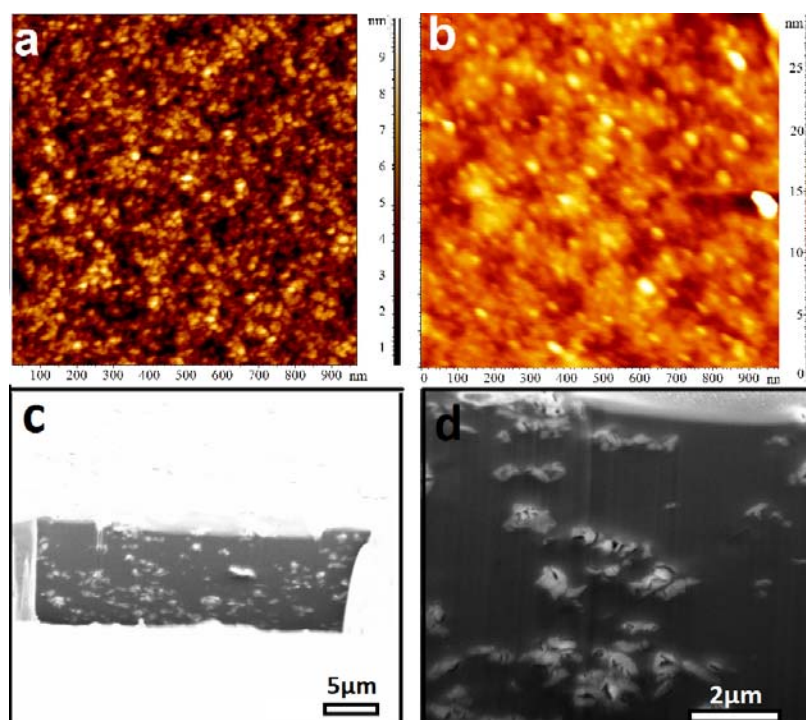
Figure 4.2 Tapping-mode AFM topographical image of the surface of a) PIMAT (9.1 wt.%) and b) PIMAT (40 wt.%); The height profile (nm) is shown for reference. FIB-SEM images of 25 wt.% \text{NH}_2\text{-MIL-53(Al)/PIMAT} (9.1 wt.%) membrane: c) the trench created by FIB milling of the specimen and d) a representative cross-section of the membrane.
