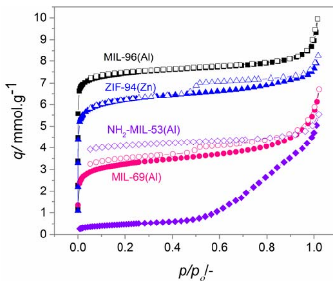
Figure 2.5 N 2 (77 K) adsorption (solid symbols) and desorption isotherms (open symbols) for the MOF materials. The absolute pressure was transferred from the relative pressure.
