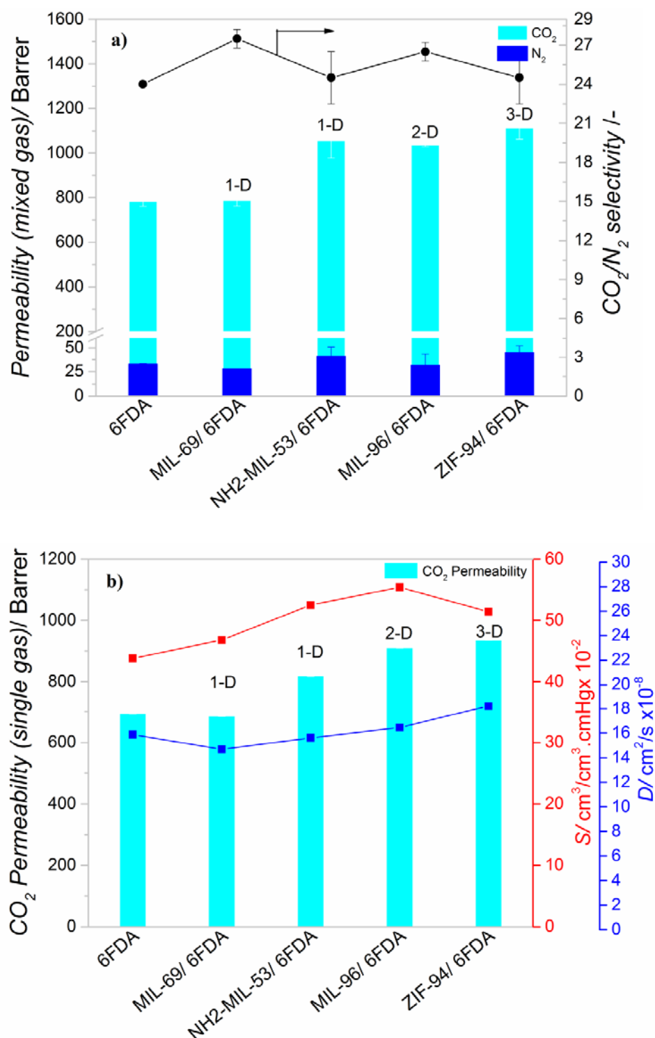
Figure 2.12 CO 2 / N 2 mixed gas separation performance of 6FDA-DAM based membranes at 298 K and 2 bar absolute feed pressure (a). Single gas CO 2 permeability, solubility and diffusivity of 6FDA-DAM based membranes at 295 K and 1 bar absolute feed pressure (b). Error bars correspond to standard deviation of duplicate membranes.
