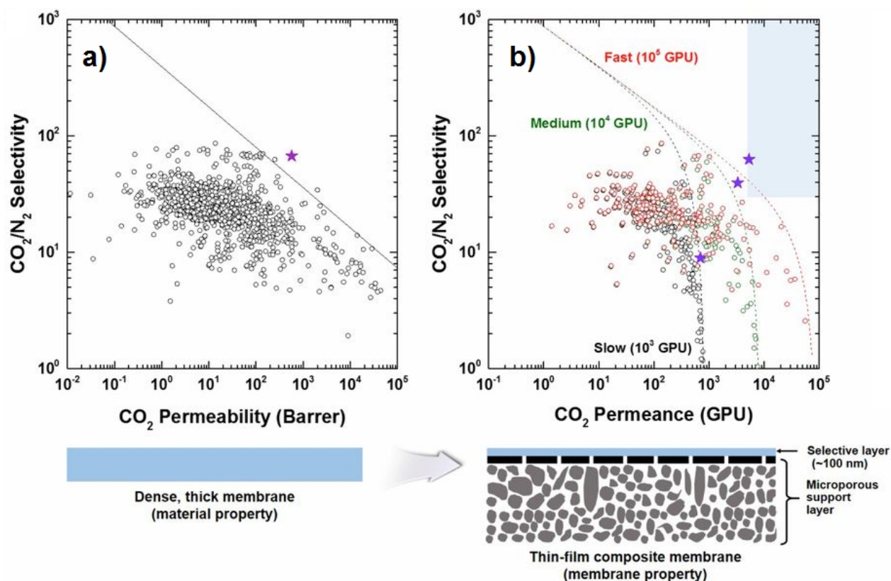
Figure 1.6. Robeson upper-bound data for \text{CO}_2/\text{N}_2 separation (a) and its translation into selectivity versus permeance, based on different support permeance (b). The star represents the permeability/selectivity of a hypothetical material with separation performance above the upper bound (a) and the permeance/selectivity of hypothetical thin-film composite membranes, using different supports (b), shaded region represents the post-combustion \text{CO}_2 capture target area. Reproduced from ref [8a].
