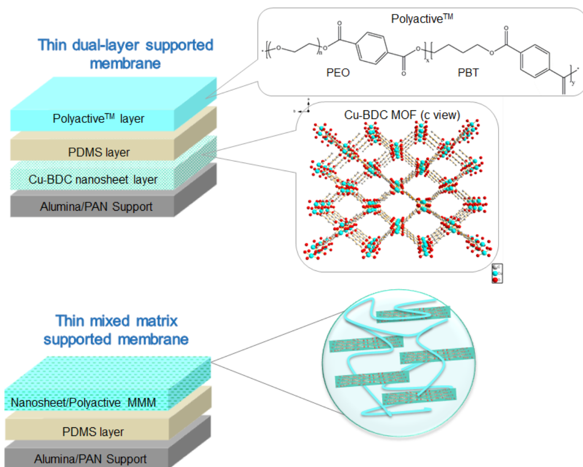
Figure 5.4. Scheme of thin supported dual layer ( top ) and mixed matrix ( bottom ) membranes prepared via dip-coating and drop-casting methods.
