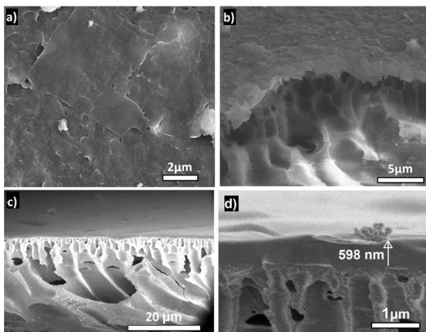
Figure 5.7. FE-SEM images of surface (a) and cross-section (b) of nanosheets coated on PAN and cross-section images of dual layer thin membranes on PAN prepared by drop-casting (ns-0.25PA-PDMS-DLM) (c, d).
