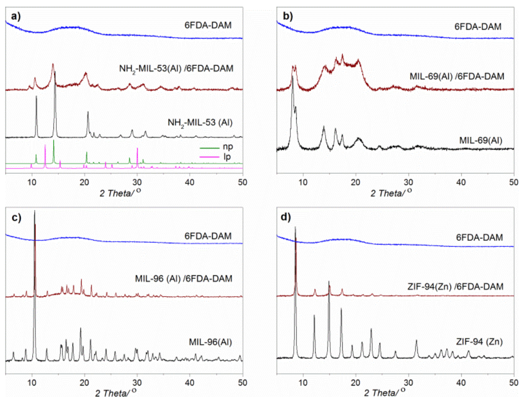
Figure 2.8 The XRD patterns of the MOF fillers, neat 6FDA-DAM membranes and MMMs. The simulated XRD patterns of \text{NH}_2\text{-MIL-53(Al)} ( lp and np forms) are shown for reference.
