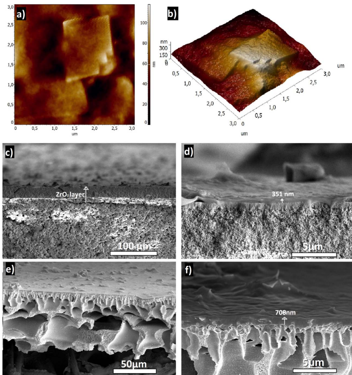
Figure 5.6. AFM 2D and 3D topography images (a, b) and FE-SEM images of thin MMMs on \text{ZrO}_2 -alumina (c, d) and PAN support (e, f) prepared by dip-coating in the mixture of 8 wt.% nanosheet in Polyactive TM (8ns-3PA-MMM).
