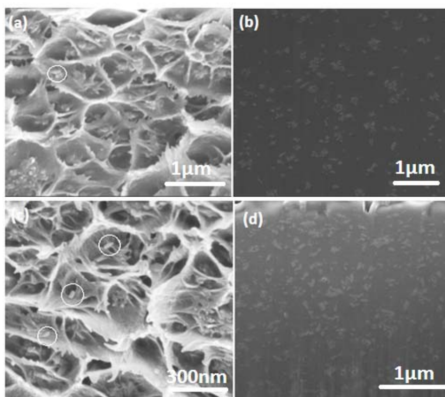
Figure 3.9 SEM micrographs of MMMs comprising \text{NH}_2\text{-MIL-53(Al)} nanoparticles and 6FDA-DAM showing a, c) cross section of the membranes prepared by freeze fracturing without FIB milling for 5 and 15 wt% MOF loadings; and b, d) cross section of the composite membrane exposed via FIB milling for 5 and 15 wt% MOF loadings.
