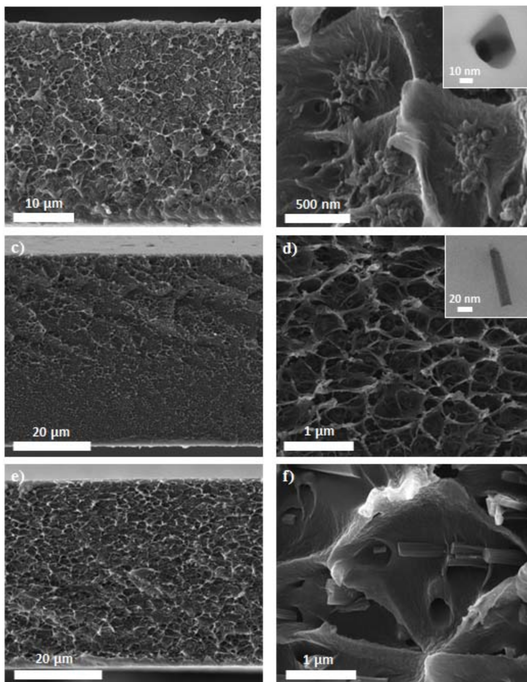
Figure 3.5 SEM images of 8 wt% NH 2 -MIL-53(Al)@Matrimid ® MMMs synthesized using the three different crystal morphologies: a, b) nanoparticles (NP), c, d) nanorods (NR) and e, f) microneedles (MN). Inset: TEM micrographs of a particle embedded in Matrimid ® acquired for the b) 8 wt% NP-NH 2 -MIL-53(Al)@Matrimid ® and d) 8 wt% NR-NH 2 -MIL-53(Al)@Matrimid ® MMMs.
