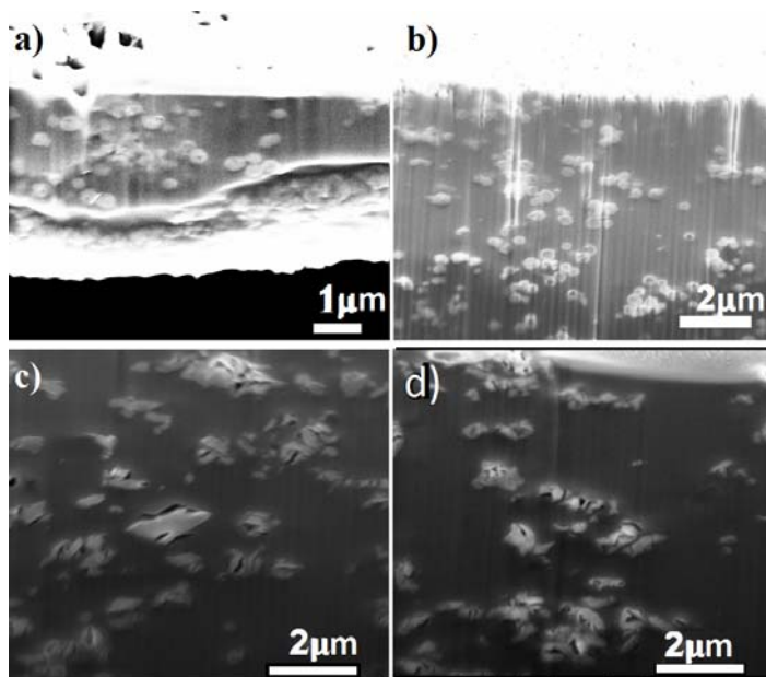
Figure 4.5. Cross-section FIB-SEM images of \text{ZIF-94(Zn)/PIM-1} (a), \text{ZIF-94(Zn)/PIMAT} (b), \text{NH}_2\text{-MIL-53(Al)/PIM-1} (c), and \text{NH}_2\text{-MIL-53(Al)/PIMAT} (d).
