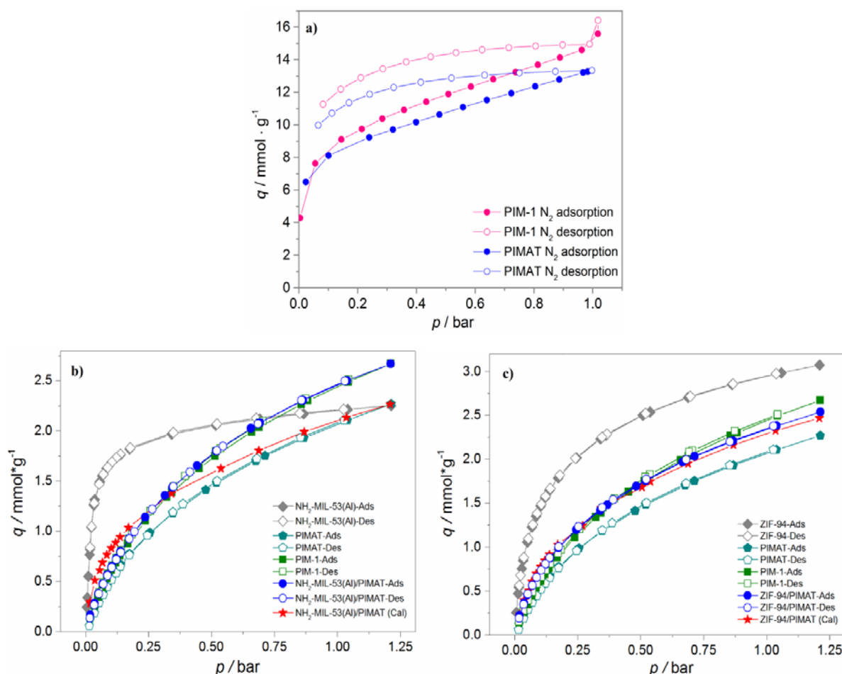
Figure 4.6 Experimental N_2 adsorption (solid symbols) and desorption (open symbols) isotherms of PIM-1 and PIMAT membranes at 77 K (a), Experimental \text{CO}_2 adsorption (solid symbols) and desorption (open symbols) isotherms of \text{NH}_2\text{-MIL-53(Al)} and membranes at 273 K (b), Experimental \text{CO}_2 adsorption (solid symbols) and desorption (open symbols) isotherms of ZIF-94(Zn) and membranes at 273 K (c). The MOF particle loading in PIMAT is 25 wt.%. The Matrimid ® loading in PIM-1 is 9.1 wt.%. The calculated isotherm is gained from a linear combination of the isotherms of \text{NH}_2\text{-MIL-53(Al)} and PIMAT based on their weight contribution.
