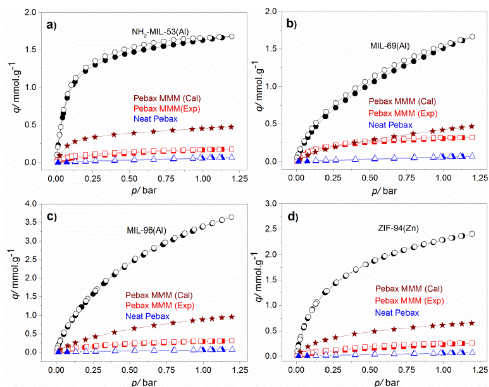
Figure 2.11 Experimental CO 2 adsorption (solid symbols) and desorption (open symbols) isotherms of MOF fillers, neat Pebax membrane and MMMs with filler loadings of 25 wt. % at 295 K. The calculated adsorption isotherms of MMMs are shown for comparison.
