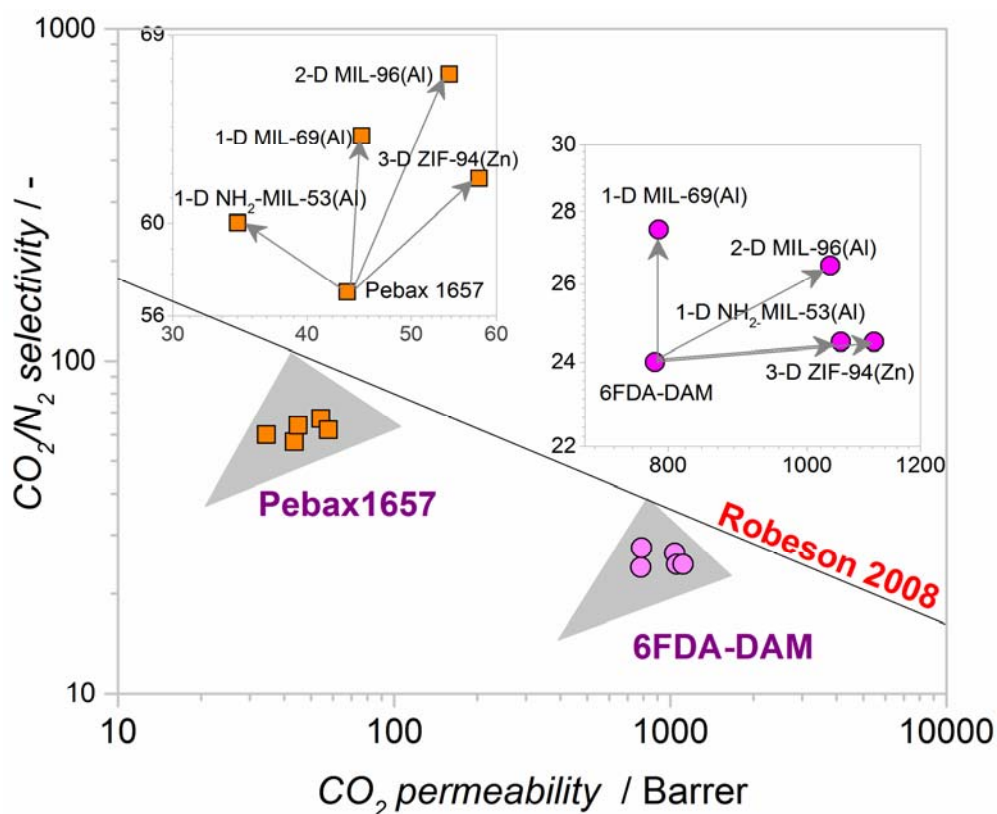
Figure 2.14. Robeson plot of \text{CO}_2 / \text{N}_2 separation performance of MOF-MMMs and neat 6FDA-DAM and Pebax membranes at 298 K and 2 bar absolute feed pressure (mixed gases). The insets are the enlarged views of the corresponding membrane performance beneath. The Robeson upper bound (2008) is shown for reference. The loading of MOFs in all the MMMs is 25 wt. %.
