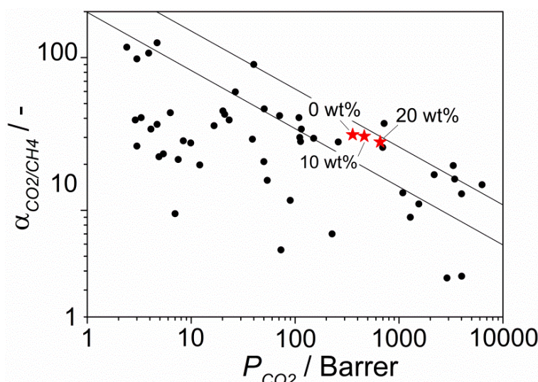
Figure 3.12 Robeson plot for the separation of CO 2 from CH 4 showing the gas separation performance of pure 6FDA-DAM and of the MMMs prepared with 10 and 20 wt% of NH 2 -MIL-53(Al) nanoparticles measured for a 1:1 CO 2 /CH 4 mixture at 298 K and \Delta p = 3 bar. Most relevant results reported in literature for MOF-based MMMs have also been included for comparison.
