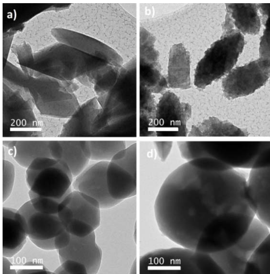
Figure 2.4 TEM images of a) \text{NH}_2\text{-MIL-53(Al)} , b) \text{MIL-69(Al)} , c) \text{MIL-96(Al)} and d) \text{ZIF-94} .
