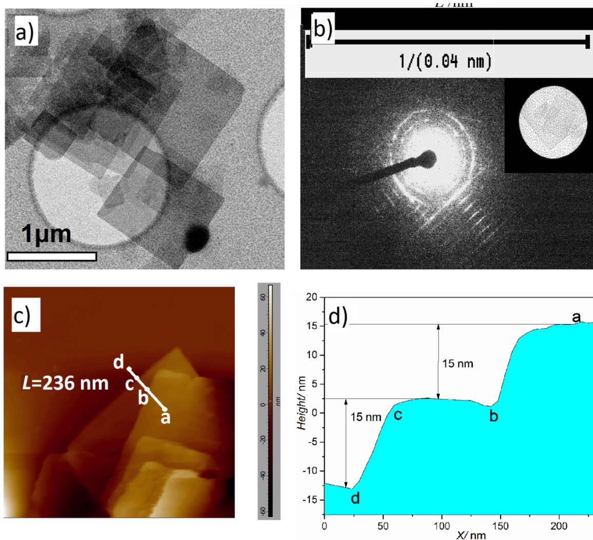
Figure 5.2. TEM images and electron diffraction pattern of region shown in inset (a, b), AFM image showing the thickness of Cu-BDC nanosheets (c, d).
