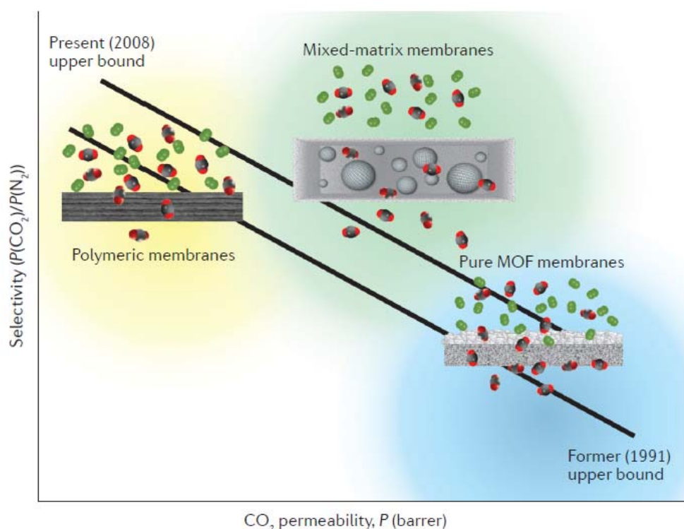
Figure 1.5. CO 2 and N 2 selectivity versus CO 2 permeability of pure polymeric, mixed-matrix, and pure MOF membranes versus Robeson upper bound. Reproduced from ref [43]
