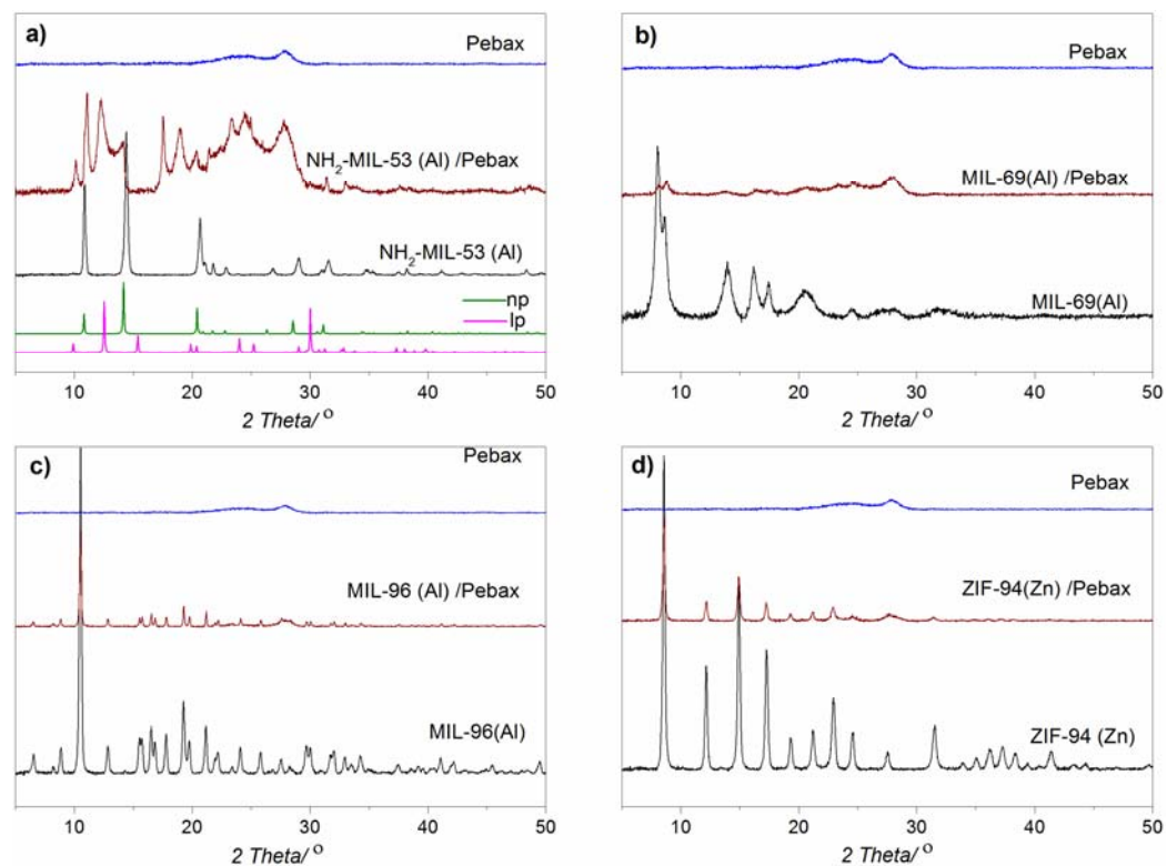
Figure 2.9 The XRD patterns of the MOF fillers, neat Pebax membranes and MMMs. The simulated XRD patterns of \text{NH}_2\text{-MIL-53(Al)} ( lp and np forms) are shown for reference.
