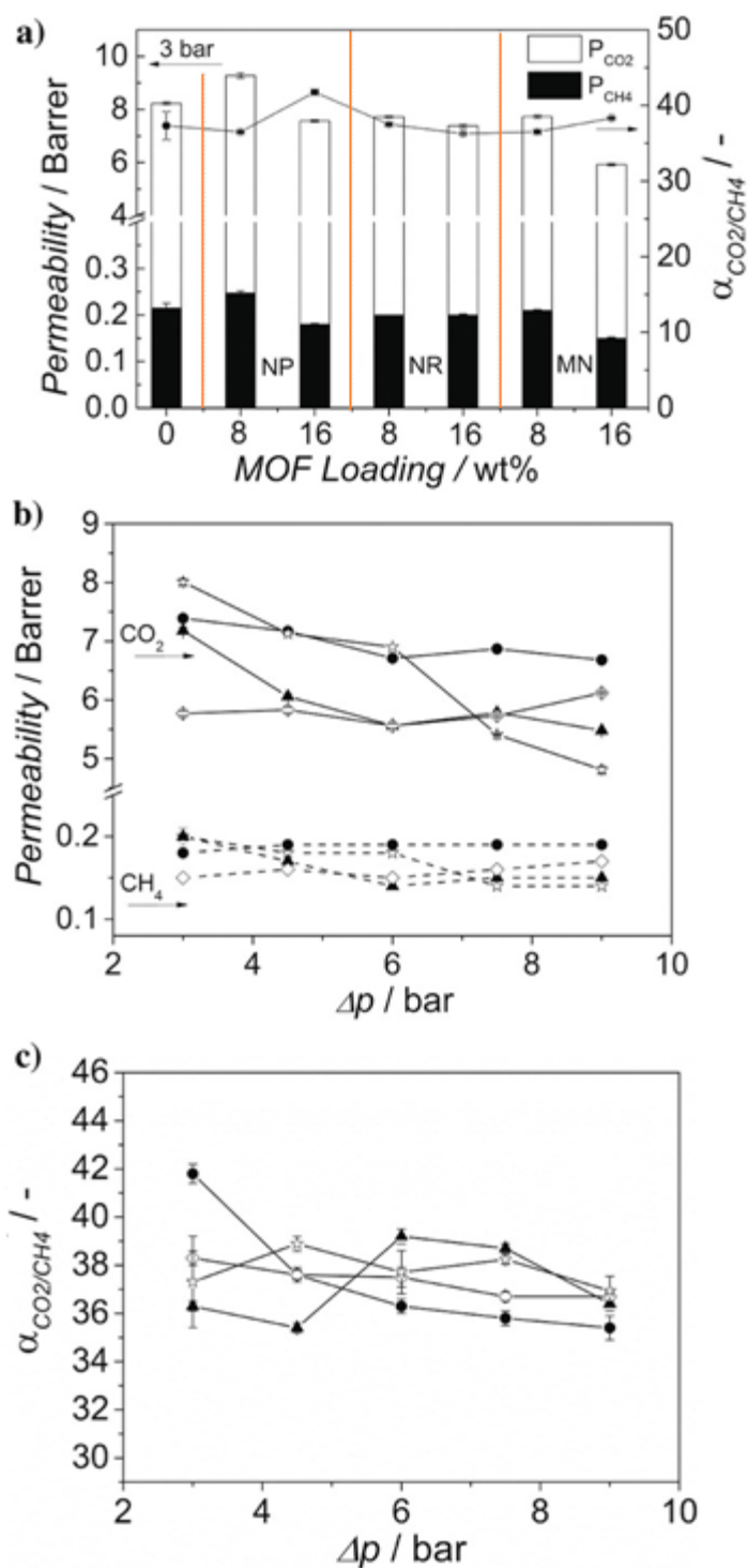
Figure 3.6. a) Permeation properties for the CO 2 /CH 4 mixture (1:1) separation at 298 K and \Delta p = 3 bar for MMMs comprising Matrimid® and NH 2 -MIL-53(Al) MOF crystals with different morphologies (nanoparticles (NP), nanorods (NR) and microneedles (MN)) as a function of the filler loading. Effect of the trans-membrane pressure different on the b) CO 2 permeability and c) CO 2 /CH 4 separation factor of the 16 wt% NH 2 -MIL-53(Al)@Matrimid® MMMs prepared with different filler morphologies. The data are average values of at least two membranes and error bars correspond to standard deviation. ▲ Nanorods, ● nanoparticles, ◇ microneedles and ☆ Matrimid®.
