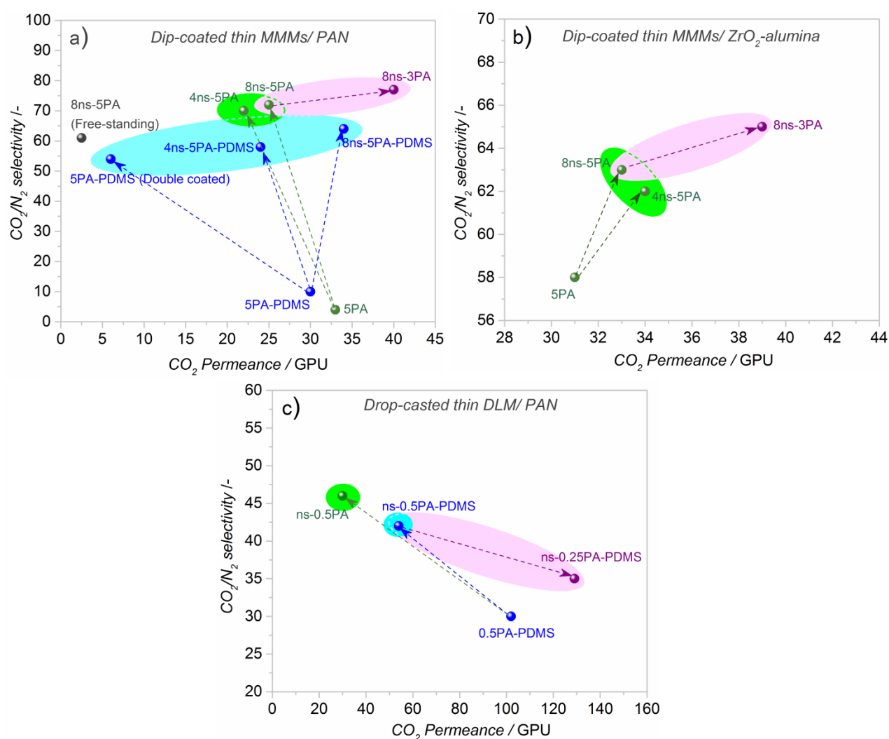
Figure 5.9. \text{CO}_2 and \text{N}_2 separation performance of dip-coated thin MMMs on (a) PAN, and (b) \text{ZrO}_2 -alumina support, (c) thin dual layer membranes drop-casted on PAN support at 298 K and 2 bar absolute feed pressure (mixed gases). In the sample identification x represents the weight percent of nanosheets based on polymer and y refers to the polymer concentration in the coating solution.
