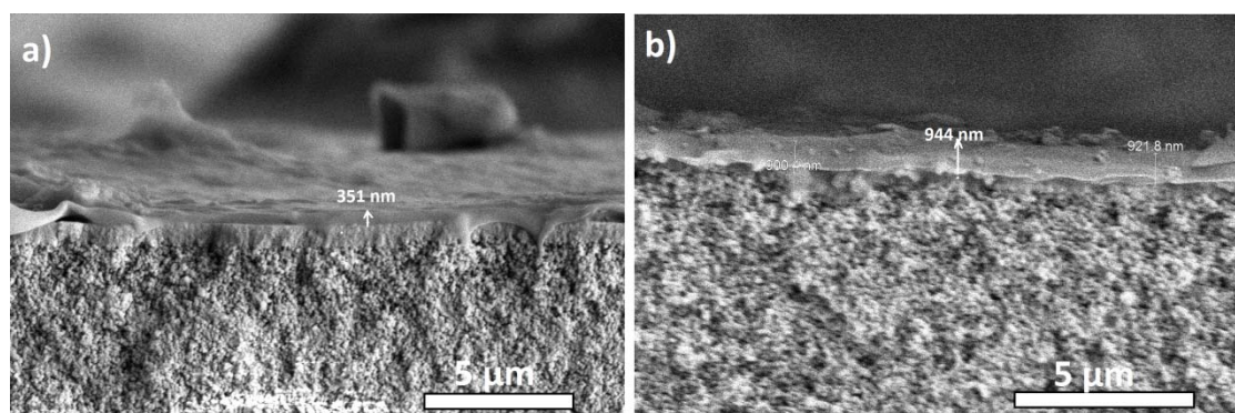
Figure 5.10. Cross-sectional FE-SEM images of thin MMMs coated on \text{ZrO}_2 -alumina prepared by dip-coating using mixture of 8 wt.% nanosheets dispersed in 3 wt.% a) and 5 wt.% b) of Polyactive™ solution (the thickness of the thin MMMs are shown).
