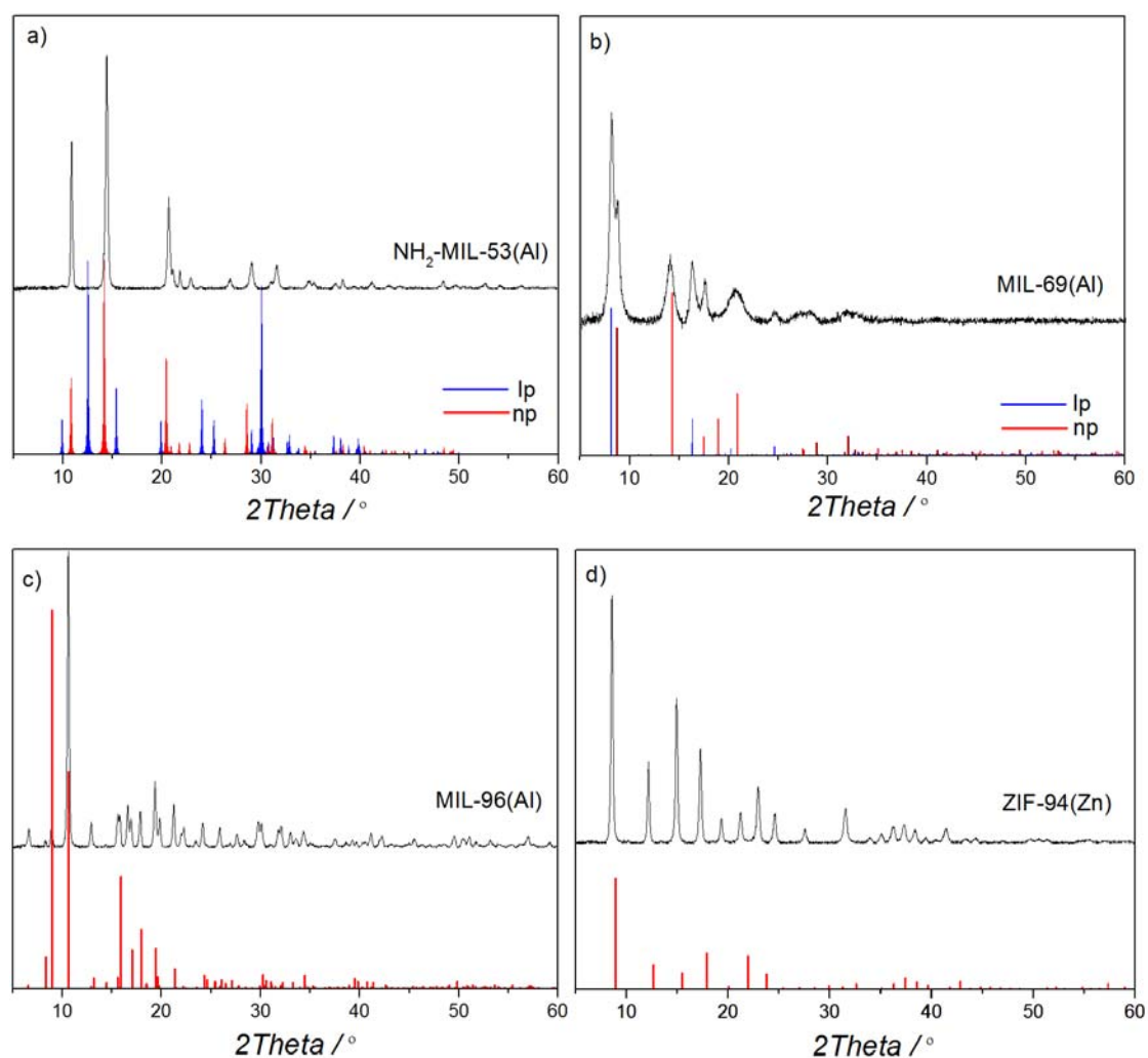
Figure 2.3 The XRD and simulated patterns of \text{NH}_2\text{-MIL-53(Al)} (a), \text{MIL-69(Al)} (b), \text{MIL-96(Al)} (c) and \text{ZIF-94(Zn)} (d).
