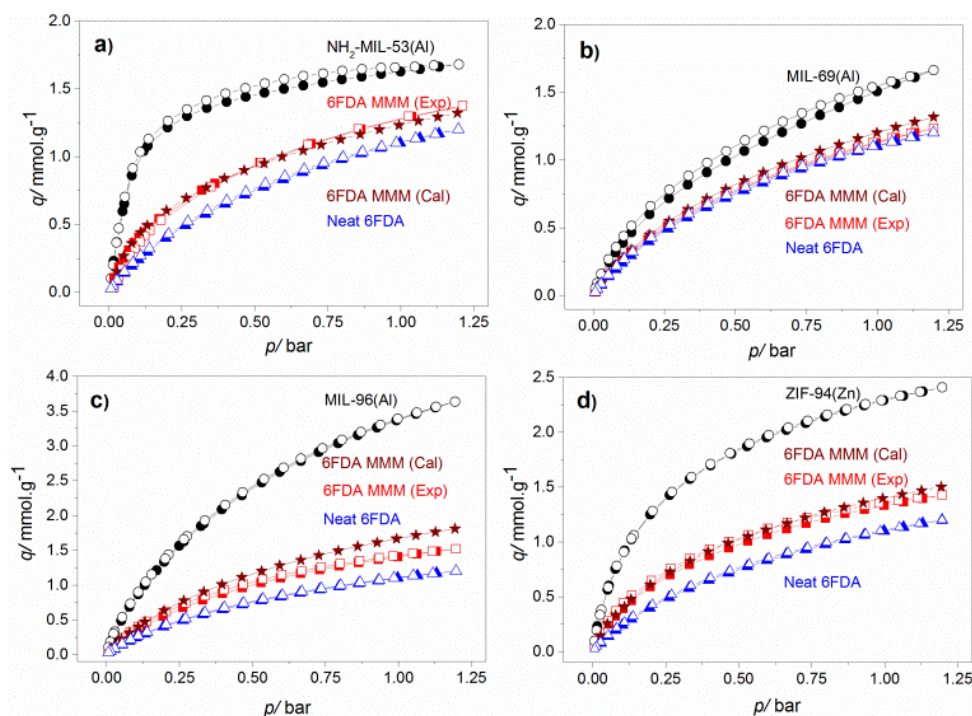
Figure 2.10 Experimental CO 2 adsorption (solid symbols) and desorption (open symbols) isotherms of MOF fillers, neat 6FDA-DAM membrane and MMMs with filler loadings of 25 wt. % at 295 K. The calculated adsorption isotherms of MMMs are shown for comparison.
