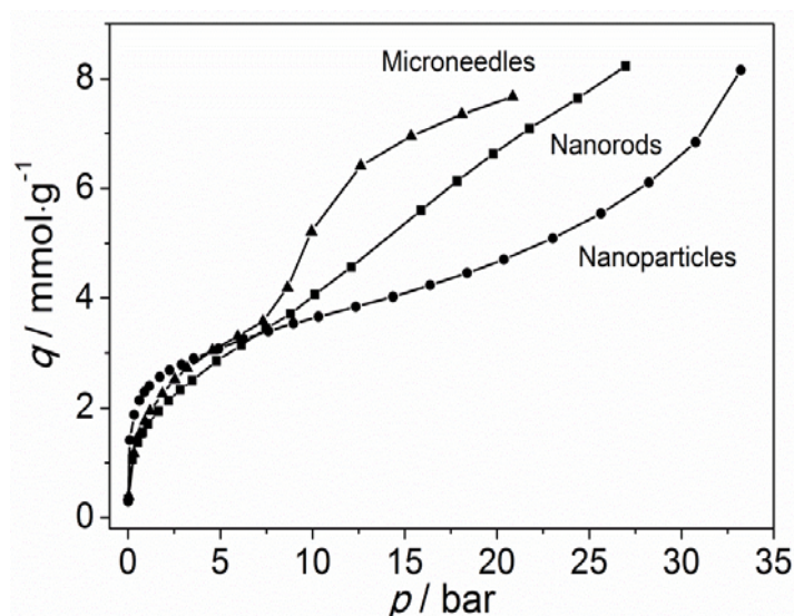
Figure 3.3 CO 2 adsorption isotherms acquired at 273 K for NH 2 -MIL-53(Al) MOF crystals with three different morphologies, i.e. nanoparticles, nanorods and microneedles.
