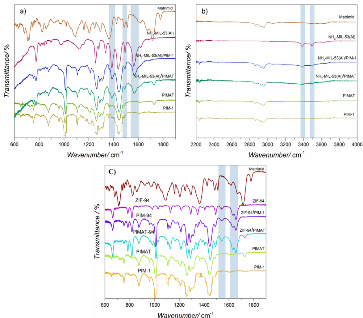
Figure 4.8 ATR-FTIR spectra of \text{NH}_2\text{-MIL-53(Al)} , PIM-1, PIMAT and MMMs between 600 and 1900\text{ cm}^{-1} (a) 2200 and 4000\text{ cm}^{-1} (b), and ATR-FTIR spectra of ZIF-94, PIM-1, PIMAT and MMMs between 600 and 1900\text{ cm}^{-1} (c).
