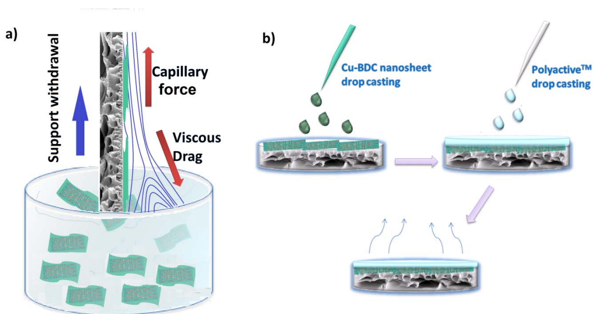
Figure 5.5. Scheme of various driving forces in dip-coating process a) and drop casting procedure b).
