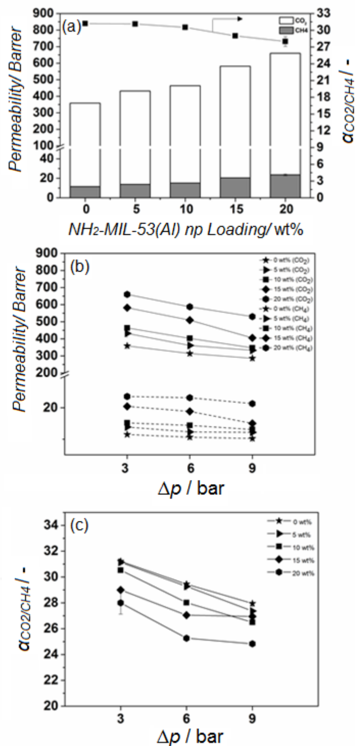
Figure 3.11 a) CO 2 and CH 4 permeation properties measured for a 1:1 CO 2 /CH 4 mixture at 298 K and \Delta p = 3 bar of MMMs comprising 6FDA-DAM and NH 2 -MIL-53(Al) MOF nanoparticles as a function of the filler loading, influence of the trans-membrane pressure difference ( \Delta p = 3, 6 and 9 bar), b) on the CO 2 permeability and c) on the selectivity of the NH 2 -MIL-53(Al)@6FDA-DAM MMMs as a function of filler loading. The data are average values of at least two membranes and error bars correspond to standard deviation. ☆ bare 6FDA-DAM and ● 5 wt%, ▲ 10 wt%, ◇ 15 wt% and ■ 20 wt% NH 2 -MIL-53(Al)@6FDA-DAM MMMs, respectively.
