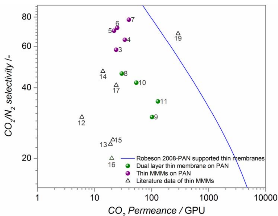
Figure 5.11. Effective Robeson limit of CO 2 / N 2 separation performance of PAN supported thin membranes ( blue line , calculation in SI) and the comparison of thin supported MMMs ( purple circles ) and dual layer membranes ( green circles ) at 298 K and 2 bar absolute feed pressure (CO 2 /N 2 mixed gases 15/85 by volume). Experimental and literature data of MOF-based thin supported and asymmetric MMMs are shown for comparison and listed in Table 2 ( open symbols ) and Table S1 ( closed symbols ).
