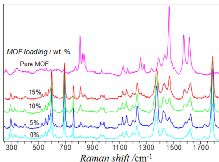
Figure 3.7 Raman spectra of bare 6FDA-DAM (labelled as “0 %”), NH 2 -MIL-53(Al) nanoparticles (labelled as “pure MOF”) and NP-NH 2 -MIL-53(Al)@6FDA-DAM MMMs with different loadings.
