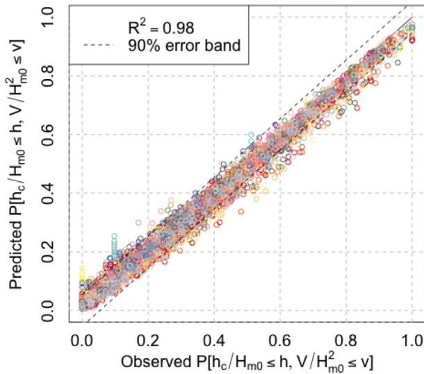
Fig. 31. Comparison between the observed and estimated non-exceedance joint probabilities for the pair h_c/H_{m0} - V/H_{m0}^2 .
