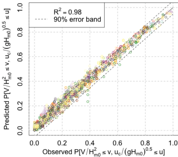
Fig. 32. Comparison between the observed and estimated non-exceedance joint probabilities for the pair V/H_{m0}^2 - u_c/\sqrt{gH_{m0}} .
