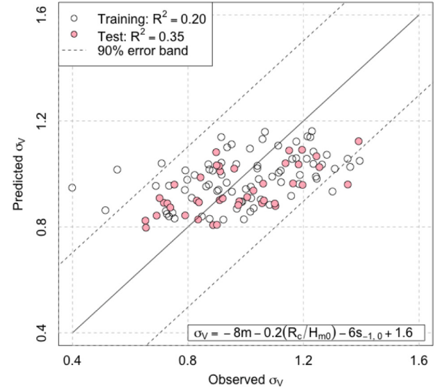
Fig. 12. Comparison between the observed and estimated \sigma_V using Eq. (12) with E_1 = -8 , E_2 = -0.2 , E_3 = -6 , E_4 = 0 and E_5 = 1.6 .
