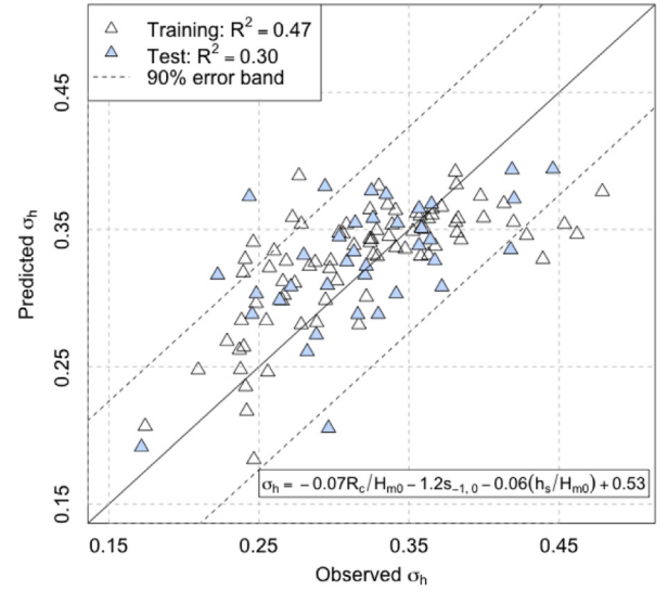
Fig. 9. Comparison between the observed and estimated \sigma_h using Eq. (6) with B_1 = 0 , B_2 = -0.07 , B_3 = -1.2 , B_4 = -0.06 and B_5 = 0.53 .
