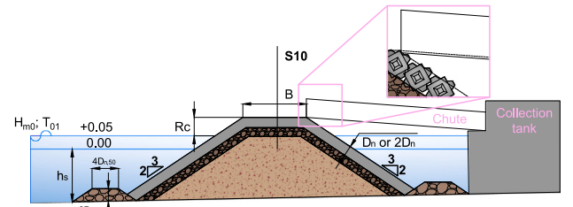
Fig. 3. Cross-section of the models tested in this study. Dimensions in m.
