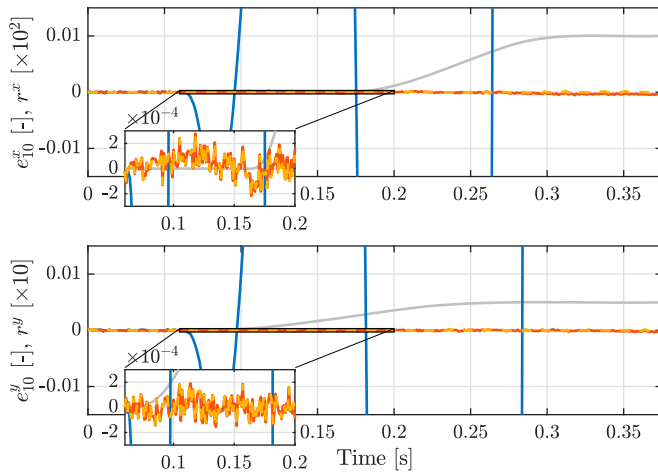
Figure 6. Error signals in trial j = 20 of the commutative SK-based approach (—), experimentally intensive approach (—), and the experimentally efficient approach (---) for the case of no model mismatch and for the scaled references trajectories r^x, r^y (---). The developed approaches achieve a significant performance gain in contrast to the commutative SK-based approach.
