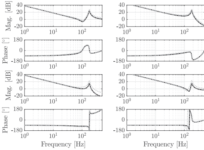
Figure 2. Bode diagram of the system P(z) used in simulation (—), and approximate model \hat{P}(z) with light (---) and severe (····) model mismatch. Clearly, the MIMO systems has interaction between inputs and outputs and is not symmetric.
