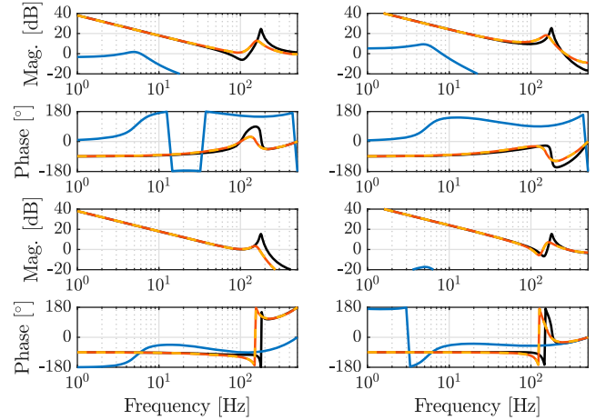
Figure 4. Bode diagram of the plant P(z) (—) and of the inverse feedforward filters \underline{F}(z, \theta_{20})^{-1} achieved with commutative SK-based approach (---), experimentally intensive approach (---), and the experimentally efficient approach (—) for the case of no model mismatch. The developed approaches approximate the system fairly well, suggesting task flexibility.
