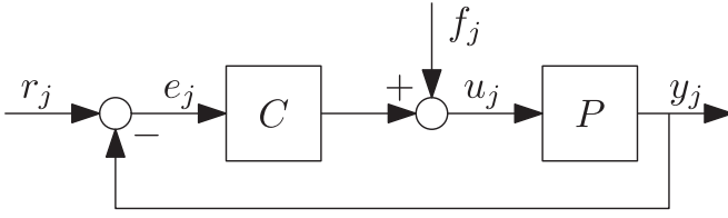
Figure 1. Closed-loop control scheme with plant P with n_i -inputs and n_o -outputs, feedback controller C , feedforward f_j and reference r_j .
