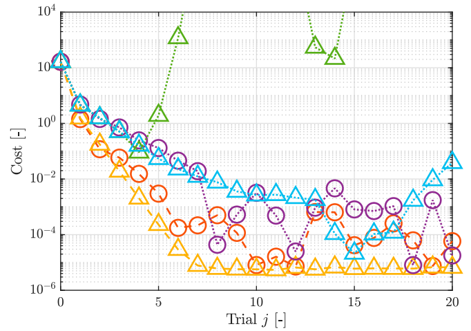
Figure 7. Error norm per trial j . The experimentally intensive approach for light ( \circ ) and severe ( \circ ) model mismatch shows that the latter converges more slowly, but still attains a low cost for certain trials without increasing regularisation. The experimentally efficient approach for severe model mismatch ( \triangle ) and for increased regularisation ( \triangle ) highlight the importance of regularisation, and the latter converges towards a slightly higher error norm, albeit at a slower rate, compared to the light model mismatch case ( \triangle ).
