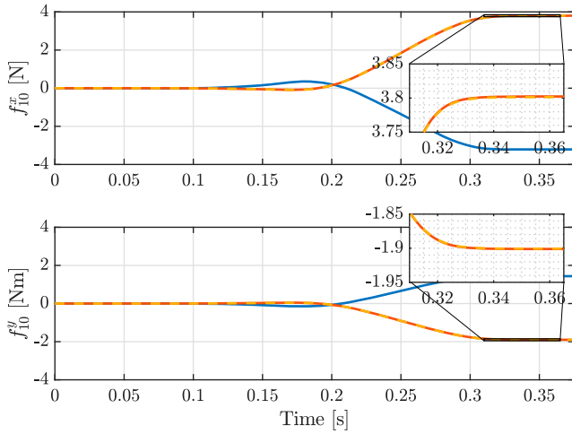
Figure 5. Feedforward signals in trial j = 20 of the commutative SK-based approach (—), experimentally intensive MIMO RBF approach (—), and the experimentally efficient MIMO RBF approach (---) for the case of no model mismatch.
