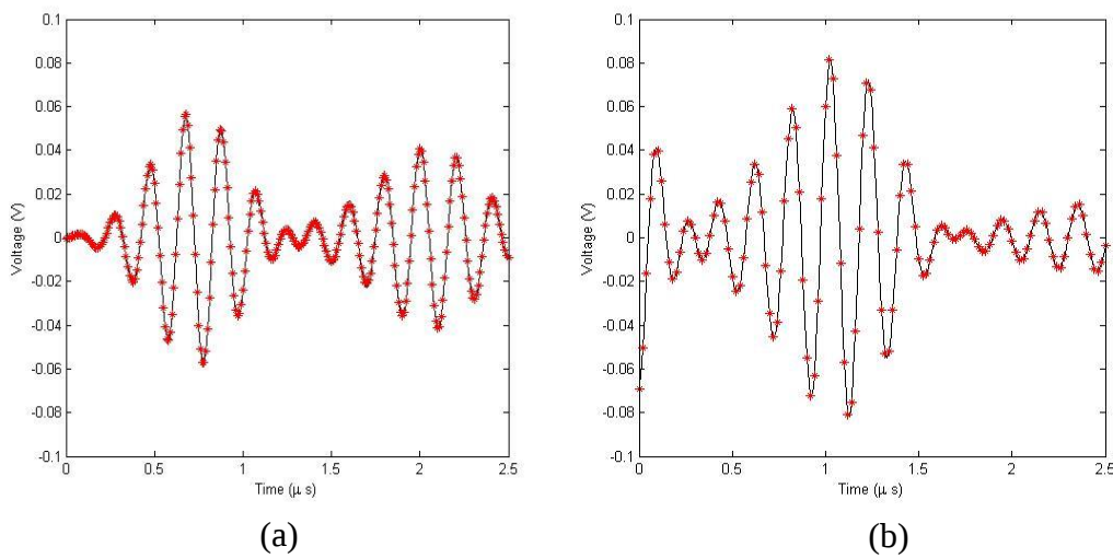
Figure 4. Model predicted signal for (a) 0.5 mm SDH (b) 2 mm SDH (Solid line: Kirchhoff approximation, Starred: Separation of Variables)
