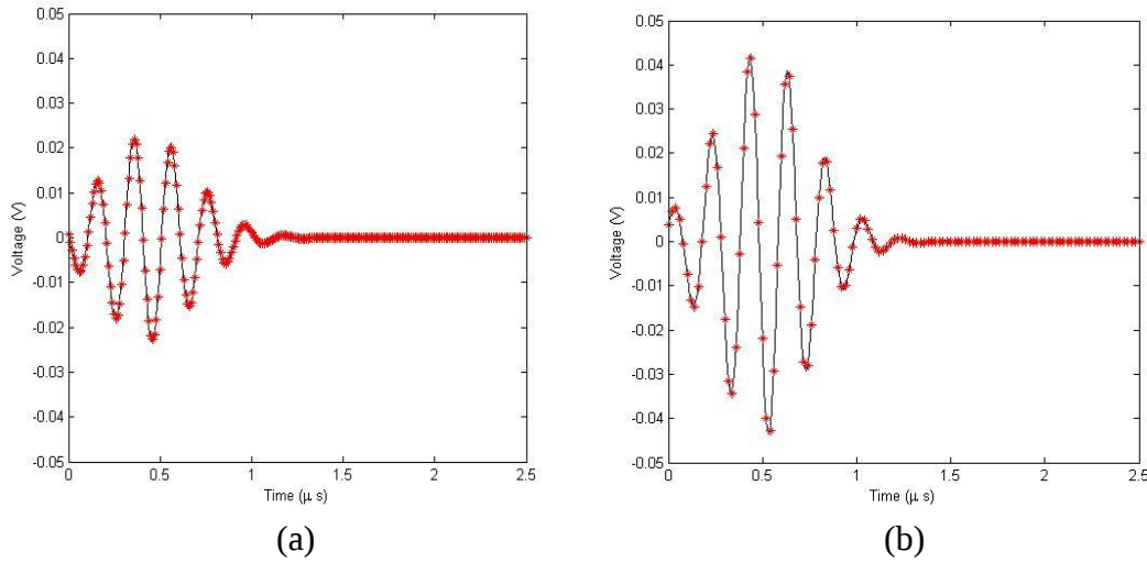
Figure 3. Model predicted signal for (a) 0.5 mm SDH (b) 2 mm SDH (Solid line: Kirchhoff approximation, Starred: Separation of Variables)
