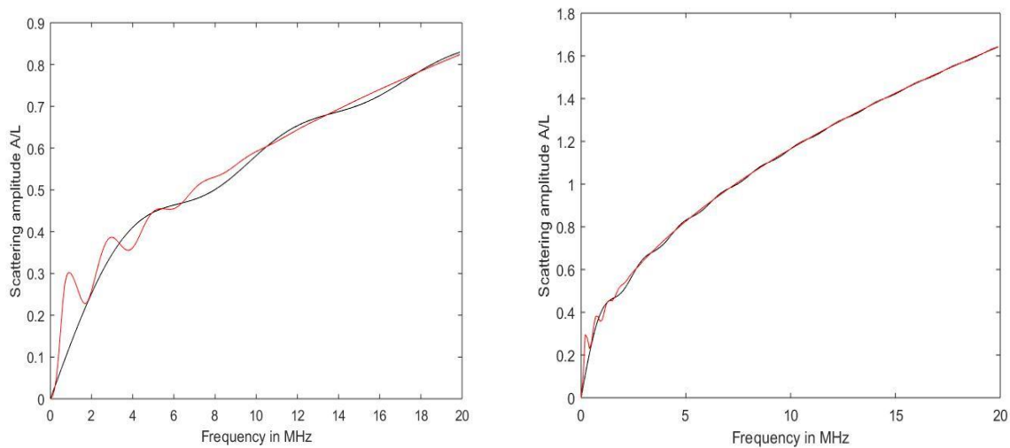
Figure 5. Scattering amplitude for (a) 0.5 mm SDH (b) 2 mm SDH (Black line: Kirchhoff approximation, Red line: Separation of Variables)
