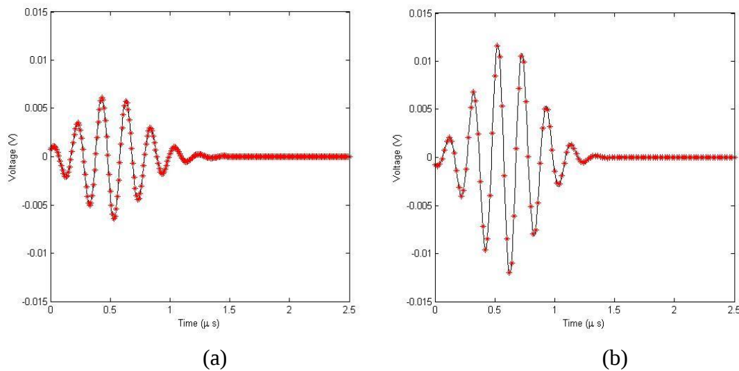
Figure 2. Model predicted signal for (a) 0.5 mm SDH (b) 2 mm SDH (Solid line: Kirchhoff approximation, Starred: Separation of Variables)
