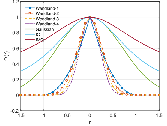
Fig. 2. Various types of global and compact (Wendland) RBF.
