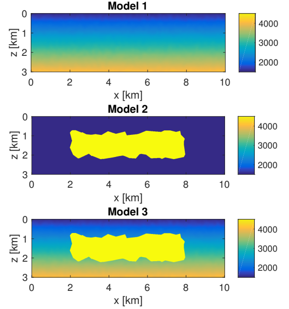
Fig. 1. Model 1: smooth velocity variation (sediment). Model 2: random 2D body with higher velocity (salt). Model 3: combination of smooth variation and blocky model. All velocities in m/s.
