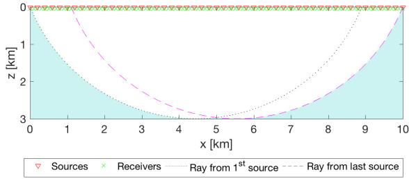
Fig. 5. Source and receivers for the simulation. Sources are placed on top, receivers at a depth of 50 m. The two ray paths separate the region recoverable by inversion from the shaded non-recoverable part [22].
