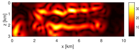
Fig. 9. Gradient of the final level set function for model A with noisy data.
