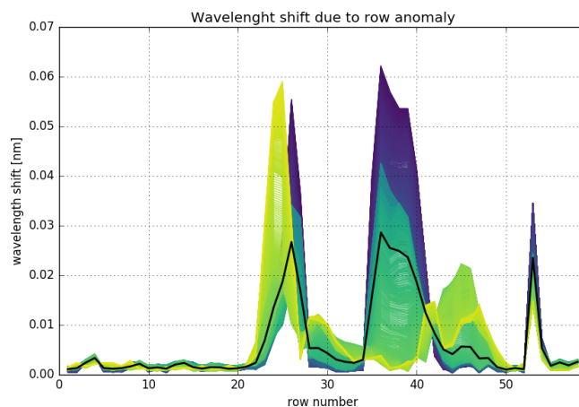
Figure 19. Radiance monitor fit wavelength shift in the VIS channel obtained from orbit 50 000. The data are averaged over all fit windows, and the absolute value is taken. Then for each measurement the moving average is determined for 100 neighboring measurements. The color scheme is the same as in Fig. 18. The result shows very high shift values for anomaly rows for most of the orbit.
