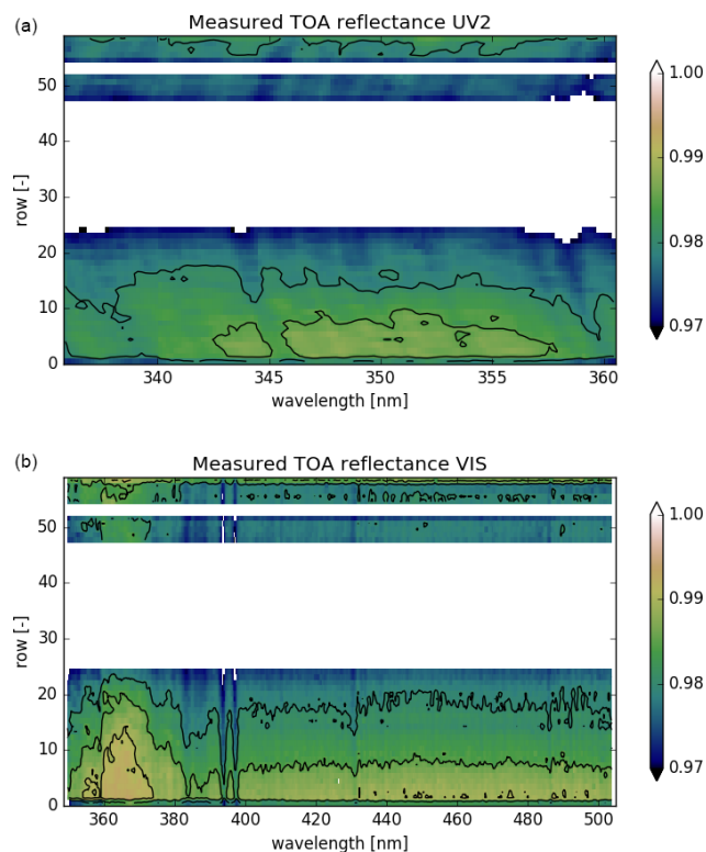
Figure 10. Averaged monthly measurements of TOA reflectances over Antarctica in January 2019 normalized to the same month in 2005 for the UV2 (a) and VIS (b) channels. Detector rows affected by the instrument row anomaly have been eliminated.
