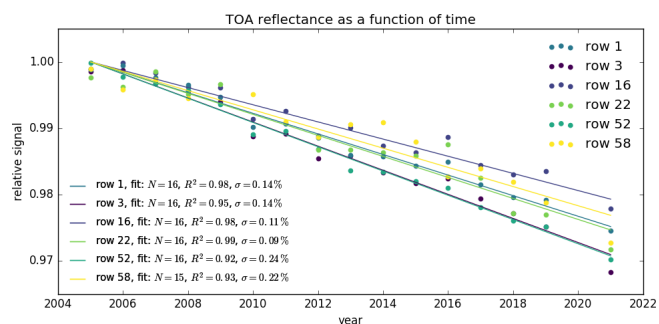
Figure 9. Changes in 340 nm TOA reflectance with time at several OMI rows over Antarctic ice surfaces. The dots show monthly averages for January, which were used to derive radiance corrections for each row individually using a linear regression model (lines). The standard deviations \sigma which are reported are for the fitting residuals.
