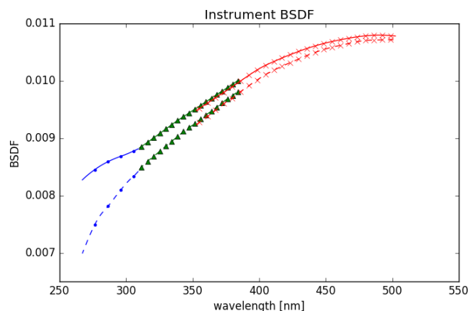
Figure 23. Instrument BSDF using the QVD for the UV1 (blue dots), UV2 (green triangles), and VIS (red crosses) channels. It can be seen that the BSDF matches quite well in the overlap regions between the bands at the start of the mission (solid line) and late in the mission (dashed line).
