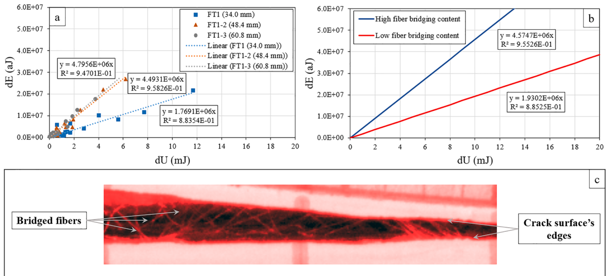
Fig. 13. Correlation of strain ( dU ) and acoustic ( dE ) energies released in FDG ( R = 0.1 ): (a) varying pre-crack lengths; (b) comparison between high (FT1-2 and FT1-3) and low bridging content (FT1, FT2, FT3, FT7, FT8, and FT9); (c) fiber bridging development.
