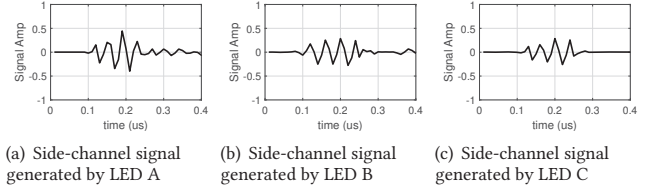
Figure 9: Observation 1: the envelopes of side-channel signals generated by LEDs of the same model are unique.
