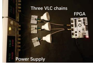
Figure 17: Centralized VLC chains/LEDs.
