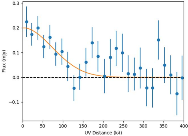
Figure 4. Visibilities (UV) profile of J13120. The UV data were extracted from the channels within the full width at zero intensity of the line from the cube and averaged in bins of 15 k \lambda . We fit the profile with a single Gaussian to estimate the intrinsic source size, finding a half-light radius of 1.20 \pm 0.15 arcseconds, consistent with the 2D elliptical Gaussian fit to the zeroth-moment map.
