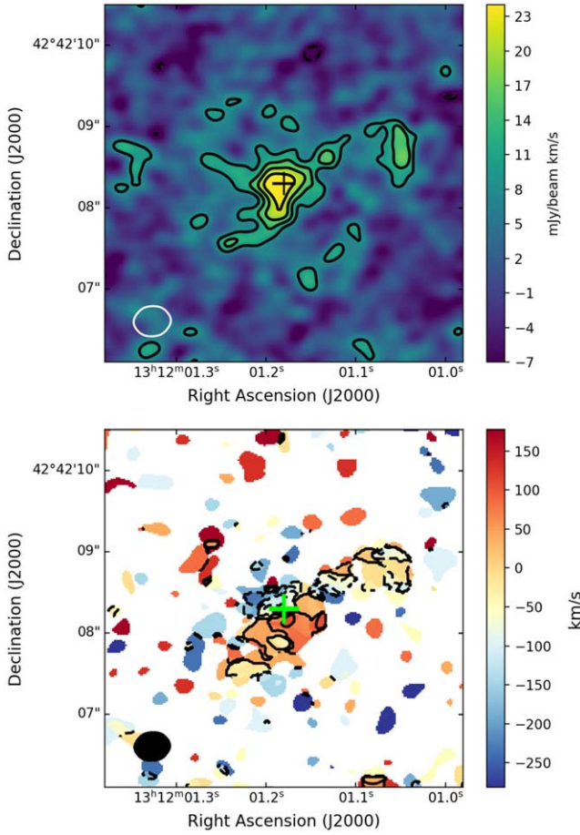
Figure 3. CO(1-0) zeroth (top) and first (bottom) moment map of SMM J13120 at a resolution of 0.39'' . The zeroth-moment map contours start at \pm 2\sigma and increase in steps of \sigma = 4.4 mJy km s ^{-1} . The first-moment map was clipped at two times the rms noise per channel ( \sigma = 9 \mu Jy beam ^{-1} ), and contours are shown in steps of 50 km s ^{-1} . We fit a 2D elliptical Gaussian to the zeroth-moment map to determine the peak position of the emission, shown by the cross, corresponding to the white cross in Figure 2.
