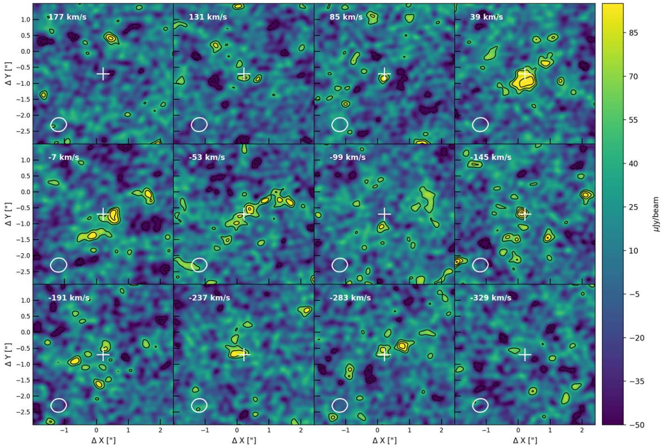
Figure 2. CO(1-0) emission maps in SMM J13120 in 46 \text{ km s}^{-1} channels. Cleaned maps are shown at a native resolution of 0''.39 from 177 km/s in the top left channel to -329 km/s in the bottom right. The shape of the beam is displayed in each channel. The white cross corresponds to the best-fit peak position of a 2D elliptical Gaussian to the zeroth-moment map. Contours start at \pm 2\sigma and increase in steps of \sigma = 27.7 \mu\text{Jy beam}^{-1} .
