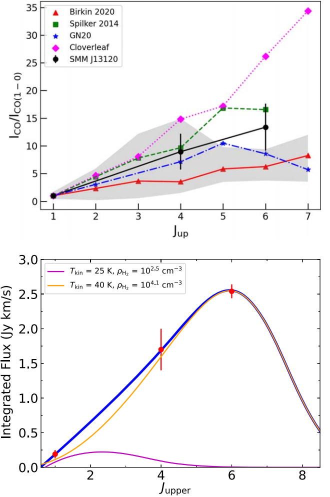
Figure 8. Top: Observed CO SLEDs normalized by the CO(1-0) flux for SMM J13120 (black circles), the SMG sample from Birkin et al. (2021, red triangles), and the SPT sample from Spilker et al. (2014, green squares). The gray shaded area represents the scatter of the Birkin et al. (2021) sample, which decreases at higher J , due to the limited number of data points. Also shown for comparison are the SMG GN20 (blue stars, Hodge et al. 2012) and the QSO Cloverleaf (magenta diamonds, Bradford et al. 2009). Bottom: CO excitation ladder (data points) and LVG model (solid line) for SMM J13120. The CO( J = 4-3 ) and CO(6-5) data points are taken from Greve et al. (2005) and Engel et al. (2010), respectively. The best fit to the data is a two-component LVG model (blue line) represented by a diffuse, low-excitation component with a kinetic temperature of T_{\text{kin}} = 25 \pm 5 \text{ K} and a gas density of \rho_{\text{H}_2} = 10^{2.5 \pm 0.1} \text{ cm}^{-3} (magenta line), and a high-excitation component with T_{\text{kin}} = 40 \pm 5 \text{ K} and \rho_{\text{H}_2} = 10^{4.1 \pm 0.3} \text{ cm}^{-3} (yellow line).
