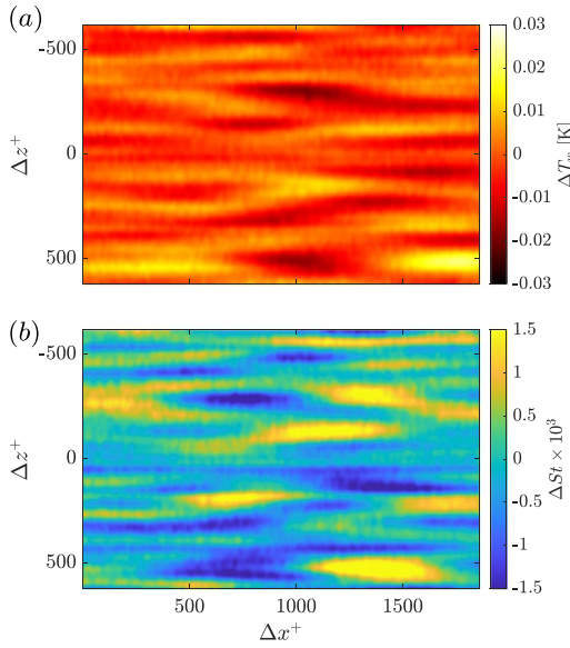
Figure 8. Instantaneous temperature map after the filtering process (a) and Stanton number map (b) from a 10 \mu\text{m} foil heated about 30 K with 3.7 V–10.0 A.
