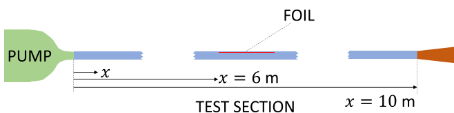
Figure 2. Sketch of the channel flow facility, with the thin foil (red) mounted on the top wall of the channel.
