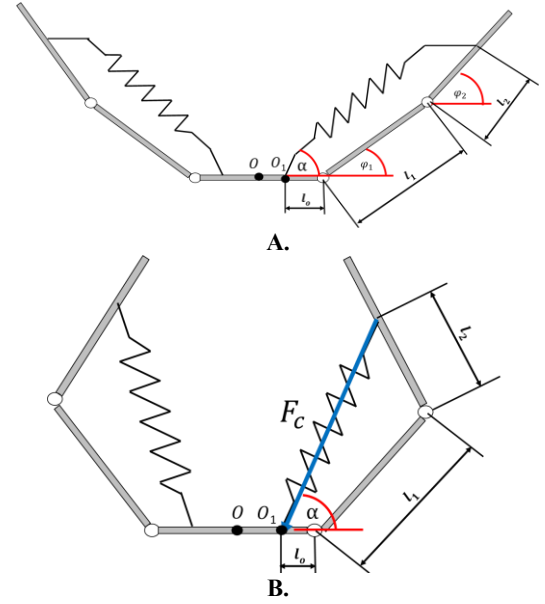
FIGURE 7: MATHEMATICAL MODEL OF THE GRASPER (A. PRESENTS POSITION BETWEEN GRASPING AND UNFOLDED MODEL B. PRESENTS THE GRASPING POSITION)
