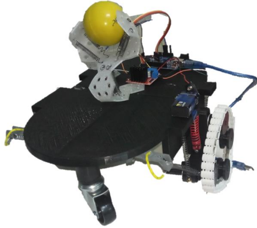
FIGURE 13: FINAL PROTOTYPE OF THE AT-GT WITH IMPLEMENTED GRASPER
