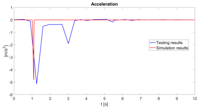
FIGURE 11: EXPERIMENTAL DATA OF ACCELERATION
