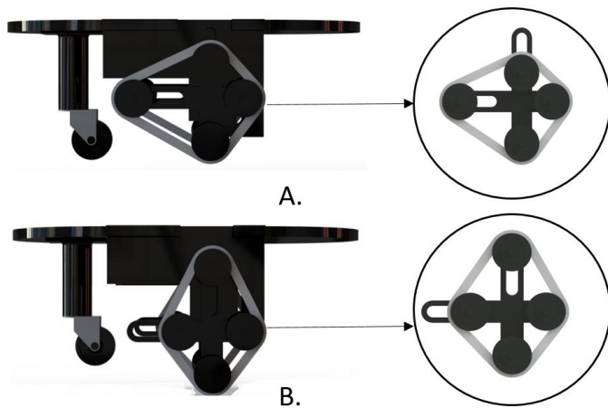
FIGURE 2: CAD MODEL OF THE AT-GT TRANSPORTER (A. LOWEST POSITION ; B. HIGHEST POSITION)
