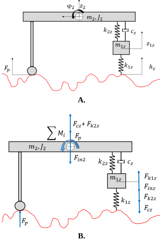
FIGURE 4: MATHEMATICAL MODEL OF THE AT-GT TRANSPORTER (A. INPUTS OF THE SYSTEM AND IT'S DOF; B. FORCES AND MOMENTS THAT INFLUECE THE RESPONSE FROM THE SYSTEM)
