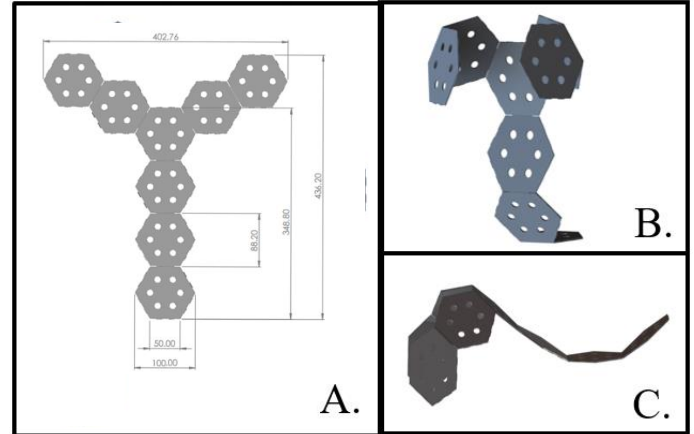
FIGURE 3: CAD MODEL OF THE GRASPER (A. THE GRASPER IN 2D (dimensions are given in [mm]); B. GRASPING; C. ROLLING/CRAWLING)
