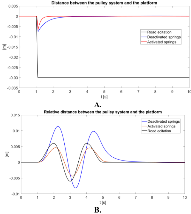
FIGURE 6: RESULTS FROM THE MATHEMATICAL MODEL SHOWING RELATIVE DISTANCE BETWEEN THE PULLEY SYSTEM AND THE PLATFORM (A. USING INPUT ON FIGURE 5. USING SINUSOIDAL ROAD PROFILE AS INPUT)
