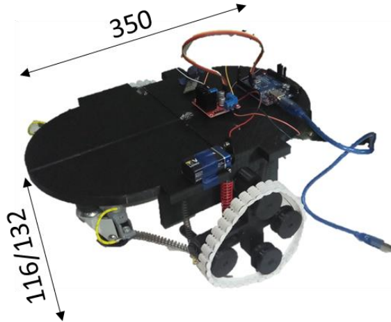
FIGURE 9: PROTOTYPE OF THE AT-GT (DIMENSIONS ARE GIVEN IN mm]
