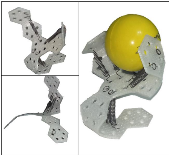
FIGURE 12: GRASPER IN SEVERAL MOVEMENTS
