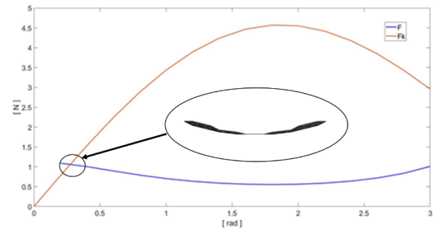
FIGURE 8: THE DEPENDENCE BETWEEN THE NECESSARY FORCE F AND THE GENERATED SPRING FORCE F_k , WHEN THE SPRING IS ACTIVATED
