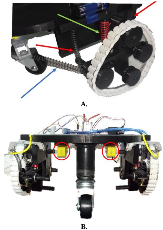
FIGURE 10: A.POSITION OF THE SMA SPRINGS; B. POSITION OF THE SERVO MOTORS
