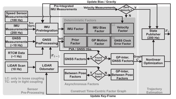
Fig. 7. System overview showing all data interfaces and factor types by implementing Algorithm 1.
