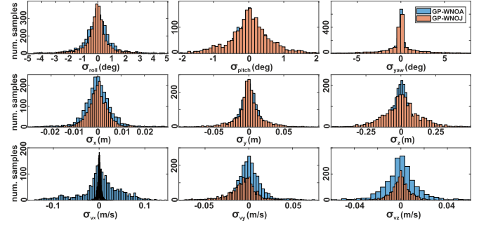
Fig. 16. Histogram of whitened state errors of GP models in an open-sky area.
