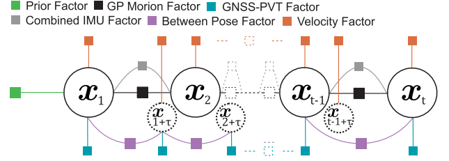
Fig. 5. General graph of loose coupling in gnssFGO.
