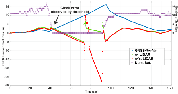
Fig. 12. Estimated GNSS receiver clock bias of Seq. C01 without near-zero-velocity detection. The receiver clock error is unobservable during tunnel crossing. In this scenario, fusing raw GNSS observations without LiDAR odometry cannot constrain the state estimation, resulting in trajectory drifting. The corresponding trajectories of both fusion approaches are presented in Fig. 11.
