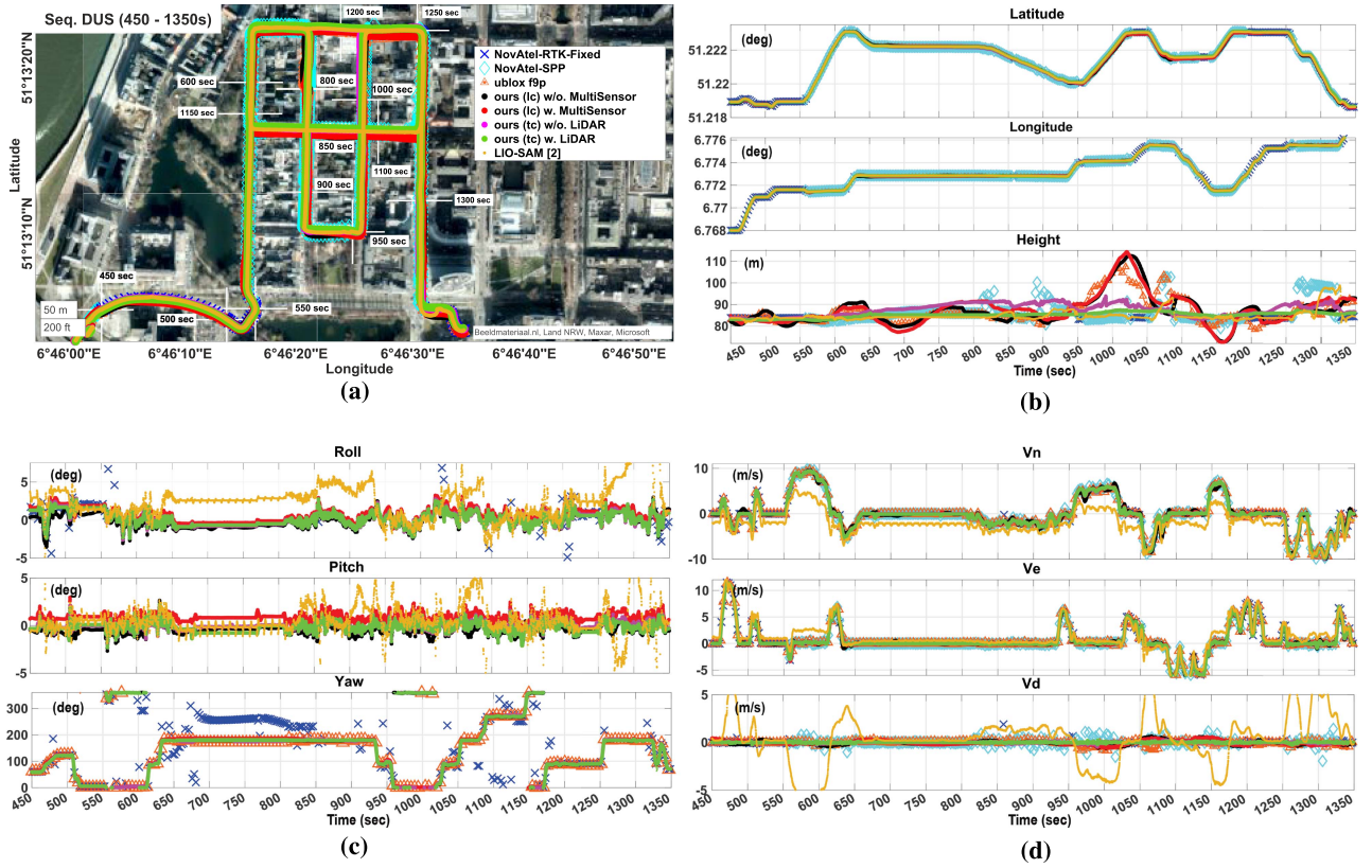
Fig. 10. Trajectory plot (450–1350 s) in challenging areas in Düsseldorf. (a) Trajectories of Seq. DUS. (b) Coordinates in the WGS84 frame. (c) Estimated rotation in the NED frame. (d) Estimated velocity in the NED frame.
