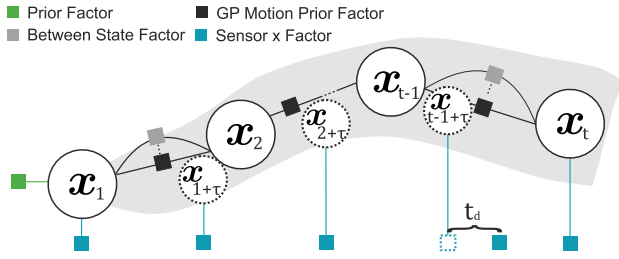
Fig. 3. General time-centric factor graph. The state variables x_t are created and constrained with GP motion prior factors on time while all asynchronous measurements are fused by querying a state with a time offset \tau between the measurement and the former state variable. The queried states (in dashed circles) are thus not to-be-estimated state variables. We assume that the measurement delay t_d is known to correct the measurement timestamp for querying a state.
