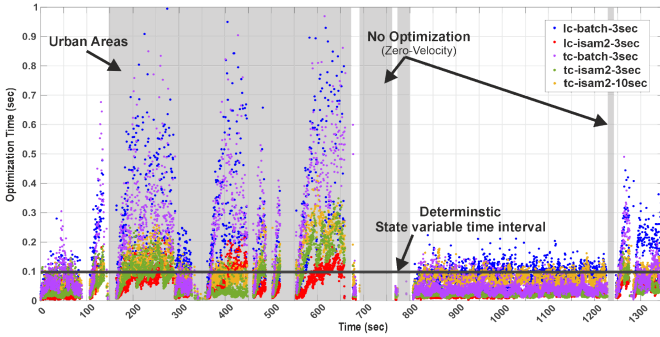
Fig. 15. Computation time with different configurations of Seq. DUS.
