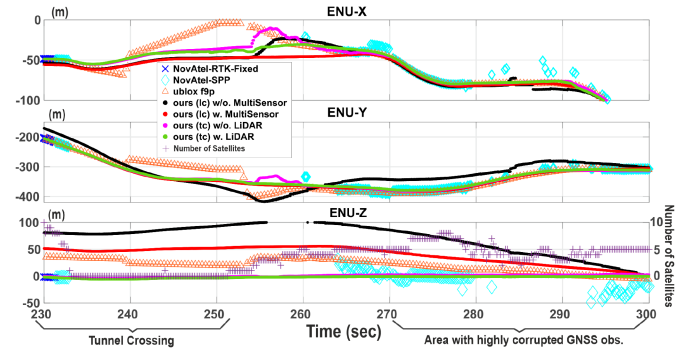
Fig. 13. Coordinates in the ENU frame of Seq. C02. The estimated trajectories become unsmooth if the GNSS observations are strongly corrupted in urban areas.
