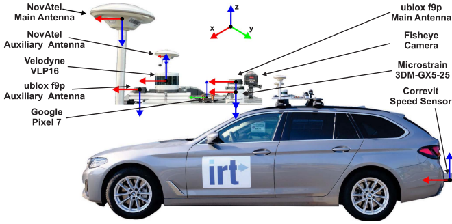
Fig. 8. Sensor setup and frames on the test vehicle.
