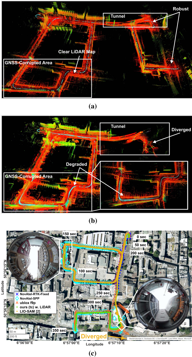
Fig. 1. Demonstration of multisensor fusion for vehicle localization of test sequence C02 in the city of Cologne. (a) LiDAR map and trajectory using tightly coupled gnssFGO (ours). The proposed method provides robust trajectory estimation and clear LiDAR maps in GNSS-corrupted areas. (b) LiDAR map and trajectory using LIO-SAM [2]. This approach fused with GNSS positioning failed due to faulty scan registrations while crossing a tunnel and degrades dramatically with corrupted GNSS measurements. (c) Measured and estimated trajectories. Fisheye images show challenging areas where GNSS observations are blocked or strongly corrupted.
