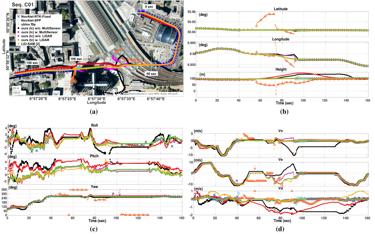
Fig. 11. Trajectory plot near the central station of Cologne (Seq. C01). For the tightly coupled fusion, we omitted the near-zero velocity detection to present trajectory drifting while the receiver clock error is unobservable. (a) Trajectories of Seq. C01. (b) Coordinates in the WGS84 frame. (c) Estimated rotation in the NED frame. (d) Estimated velocity in the NED frame.
