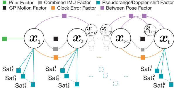
Fig. 6. General graph of tight coupling in gnssFGO with k raw satellite observations at each timestamp t denoted as \text{Sat}_t^k .
