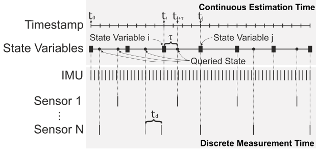
Fig. 2. Continuous-time state estimation with asynchronous measurements. A time offset \tau can be calculated with respect to a former state variable x_i at timestamp t_i for each asynchronous measurement. The variable t_d denotes a measurement delay that is assumed to be given.
