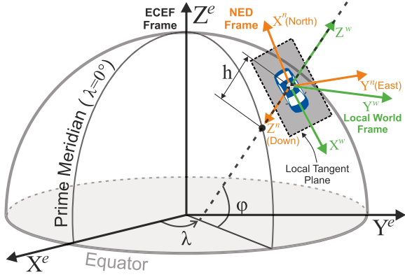
Fig. 4. Coordinate frames used in this work.
