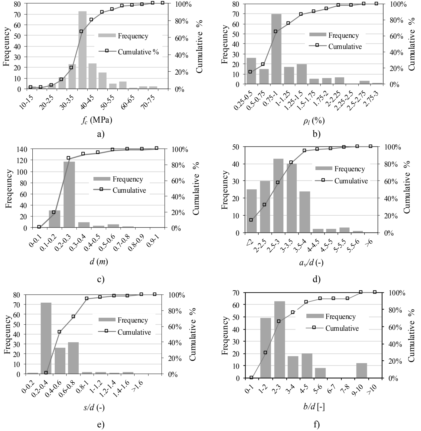
Figure 8 - Distribution of parameters in database: (a) concrete compressive strength f_c ; (b) reinforcement ratio \rho ; (c) effective depth of the longitudinal reinforcement d ; (d) clear shear span to effective depth ratio a_v/d ; (e) rebar spacing to effective depth ratio s/d ; (f) member width to effective depth ratio b/d .
