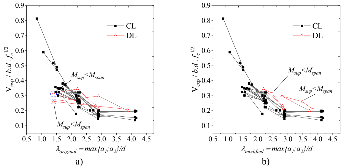
Figure 11 – Relation between experimental shear capacities and different definitions of shear slenderness \lambda : a) shear slenderness based on the ratio \max\{a_1; a_2\}/d regardless of the bending moments M_{sup} and M_{span} ; b) definition of \max\{a_1; a_2\}/d modified for continuous members under uniformly distributed loads according to M_{sup} and M_{span} .
