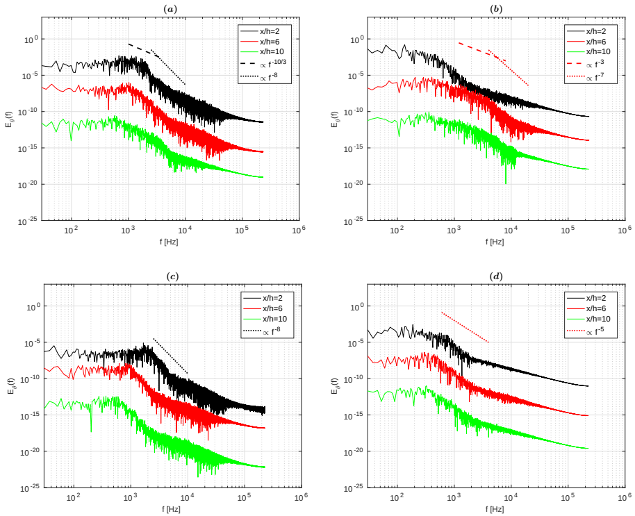
Figure 3.20: The power spectra of the temperature for Pr = 0.71 (a,b) and Pr = 0.006 (c,d) at the following monitoring point locations: y/h = 0 (a,c) and -1 (b,d) and z/h = 0 - Note that, because of readability purposes, the red and green profiles have been systematically shifted by dividing the original signals by factors 10^5 and 10^{10} , respectively.
