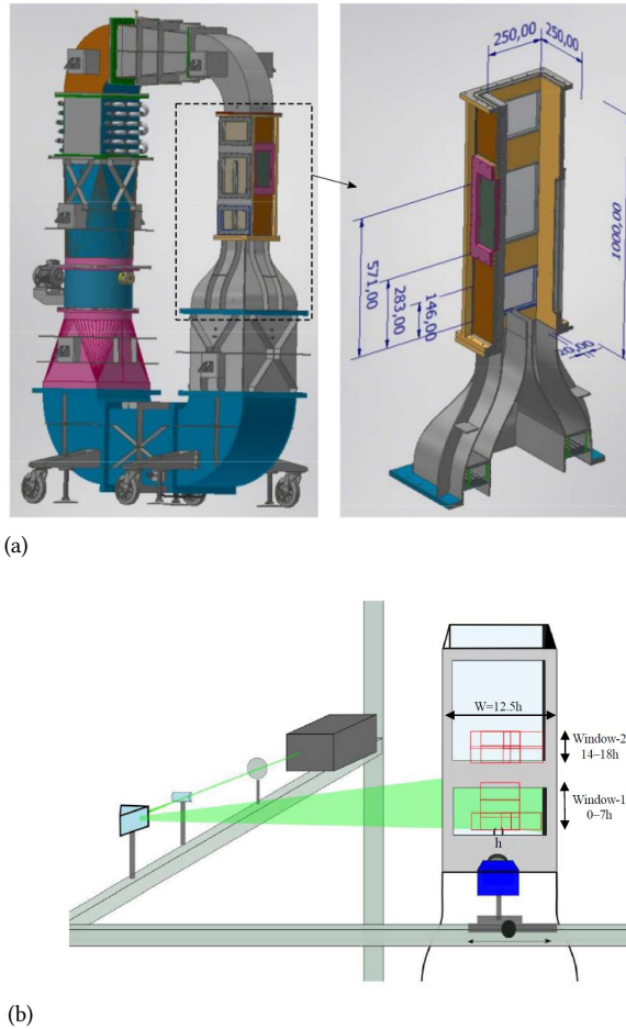
Figure 2.1: Sketch of the MYRTE wind tunnel (a) and PIV experimental set-up (b).
