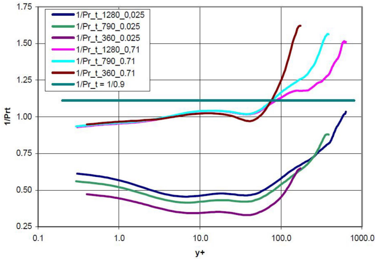
Figure 1.4: Profiles of the inverse of Pr_t from DNSs of turbulent channel flows at different friction Reynolds numbers ( Re_\tau = 360, 790, 1280 ) and Pr = 0.025 and 0.71 compared with the constant-value approach ( Pr_t = 0.9 ), [19].
