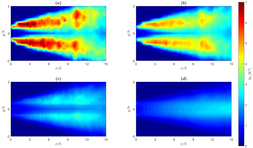
Figure 3.7: Contours of long-term time-averaged temperature variance ( k_\theta = \langle \theta' \theta' \rangle / 2 , where \theta' = \hat{T} - \langle \hat{T} \rangle ) at \text{Pr} = 0.71 (a), \text{Pr} = 0.2 (b), \text{Pr} = 0.025 (c) and \text{Pr} = 0.006 (d).
