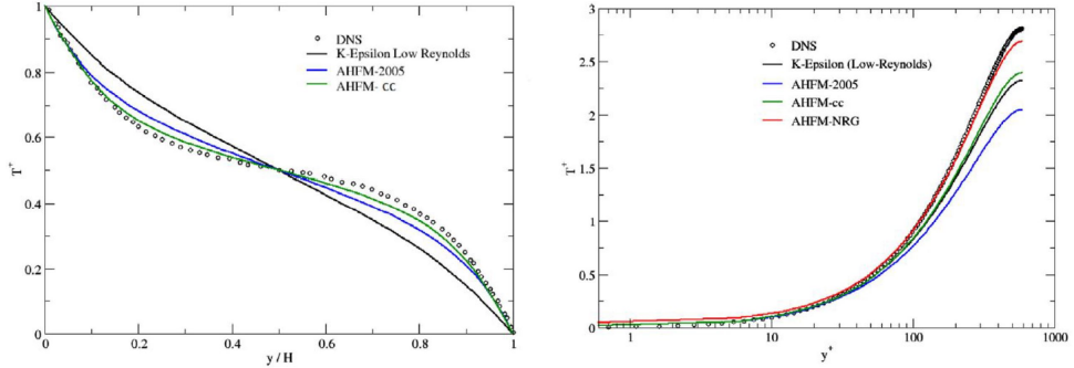
Figure 1.7: Universal temperature profiles from different low-Pr heat transfer models for Rayleigh-Bénard convection with Rayleigh number of 100000 and Pr = 0.025 (left) and channel flow (right) with Re_\tau = 590 and Pr = 0.01 , [48].
