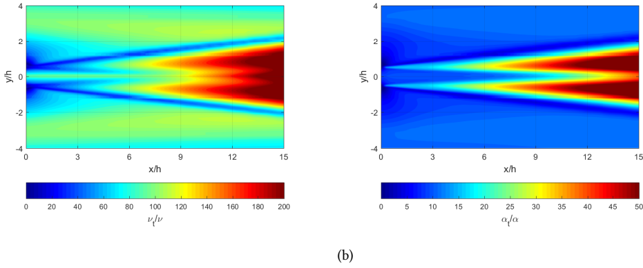
Figure 2.6: Contours of turbulent to molecular viscosity (a) and diffusivity (b) ratios at Pr = 0.2 , obtained from the low-Reynolds (k - \varepsilon - \zeta - f) + (k_\theta - \varepsilon_\theta) turbulence model (domain D2.1).
