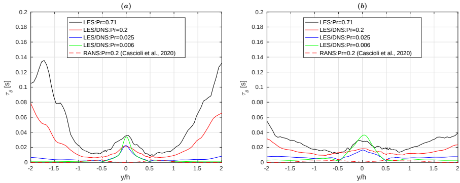
Figure 3.16: Profiles of resolved time-averaged thermal time-scale at x/h = 5 (a) and 10 (b).
