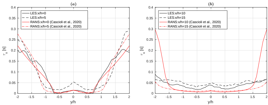
Figure 3.12: Profiles of resolved time-averaged dynamical time-scales in the convergent (a) and self-similar (b) regions of the jet.
