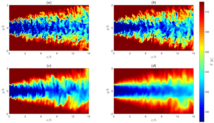
Figure 3.6: Contours of resolved instantaneous temperature ( \hat{T} ) at Pr = 0.71 (a), Pr = 0.2 (b), Pr = 0.025 (c) and Pr = 0.006 (d).
