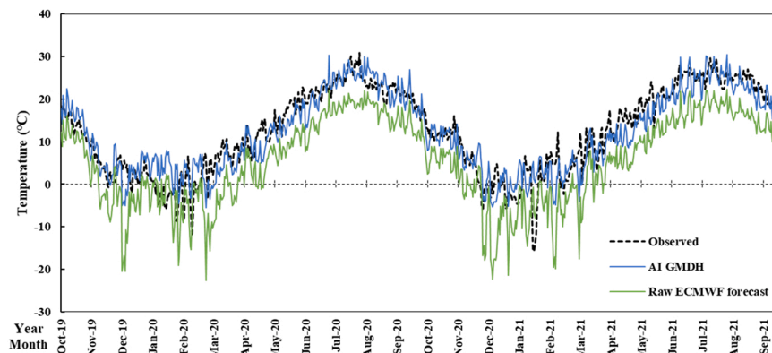
Fig. 10. Comparison of raw (ECMWF) and downscaled daily temperature forecasts at Saqez station using the GMDH downscaling method.
