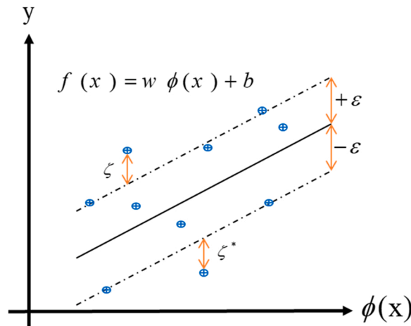
Fig. 5. The best approximation value \varepsilon to minimize the error in a specific threshold corresponds to SVR.
