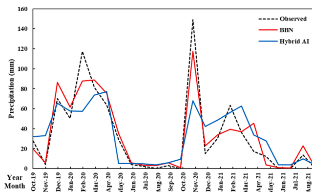
Fig. 13. Comparison of 1-month precipitation forecasts by the BBN and hybrid AI methods with observed precipitation in 2020 and 2021 at Sazez station.
