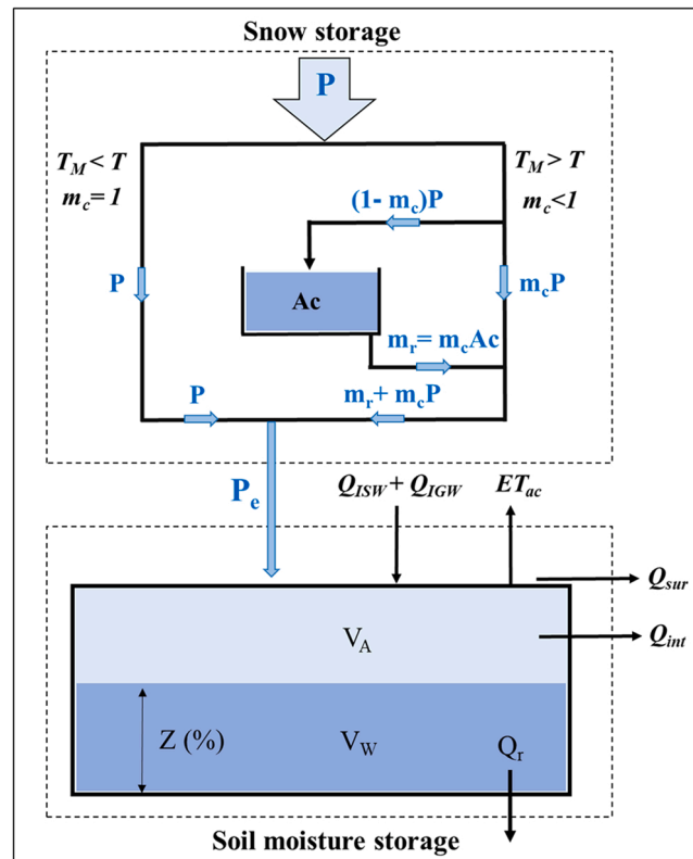
Fig. 8. Schematic diagram of the hydrological rainfall-runoff model consisting of snow and soil moisture storages. Variables are defined in Tables 3 and 4 . Each water balance component is formulated on a daily scale.
