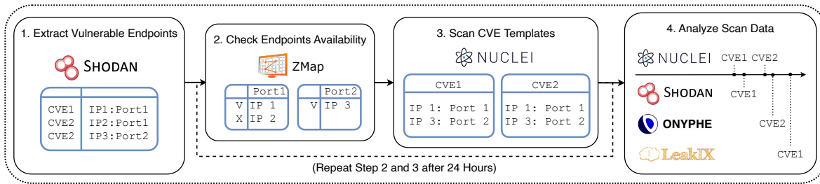
Figure 1: Research Workflow.
