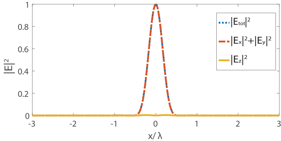
Fig. 4. Profiles of the intensities at the detector plane with a polarization convertor and a small pinhole with radius r = 0.18\mu\text{m} which is 0.36\lambda in terms of wavelength. The system is composed of: a high \text{NA}_1 = 0.9 focusing objective lens and a low \text{NA}_2 = 0.3 lens for detection. For illumination, radially polarized light of wavelength \lambda = 500\text{nm} is used. The focal field can be seen in Eq. (17). The dipole is set rigidly along the z -axis direction (only \alpha_{zz} is relevant). The plots are normalized to on-axis maxima.
