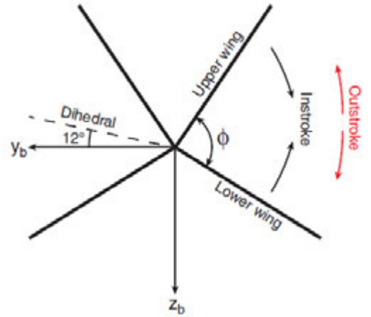
Fig. 2. Wing motion definitions.
