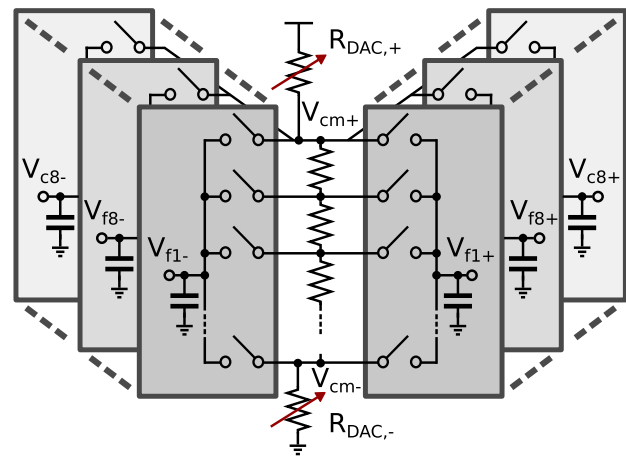
Fig. 9. Comparator calibration DAC.
