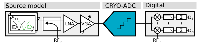
Fig. 3. System model used for specifications.
