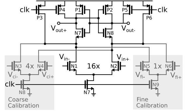
Fig. 7. Strong-arm comparator with calibration pairs.
