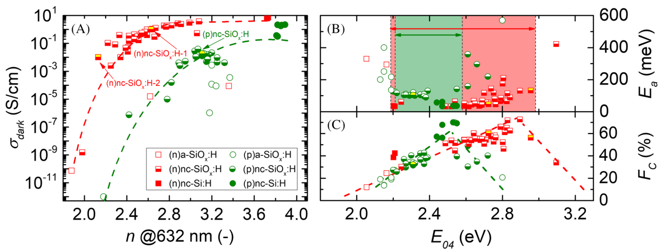
FIGURE 1 The sum-up of measured optoelectrical properties of doped nc-SiO x :H, nc-Si:H, and a-SiO x :H layers during the optimization process: (A) \sigma_{\text{dark}} vs n ; (B) E_a vs E_{04} ; (C) F_C vs E_{04} . Note: half-down symbols represent nc-SiO x :H layers; solid symbols represent nc-Si:H layers that miss CO 2 during the depositions; open symbols that distinguish a-SiO x :H are based on F_C from Raman spectroscopy; dashed lines in A,C are guides to the eye; colored rectangular areas in B indicate the optical window of achieving acceptable E_a (less than 200 meV) for solar cells application. Doped nc-SiO x :H layers that are used in fabricating solar cells are marked with labels given in Table 2 [Colour figure can be viewed at wileyonlinelibrary.com]
