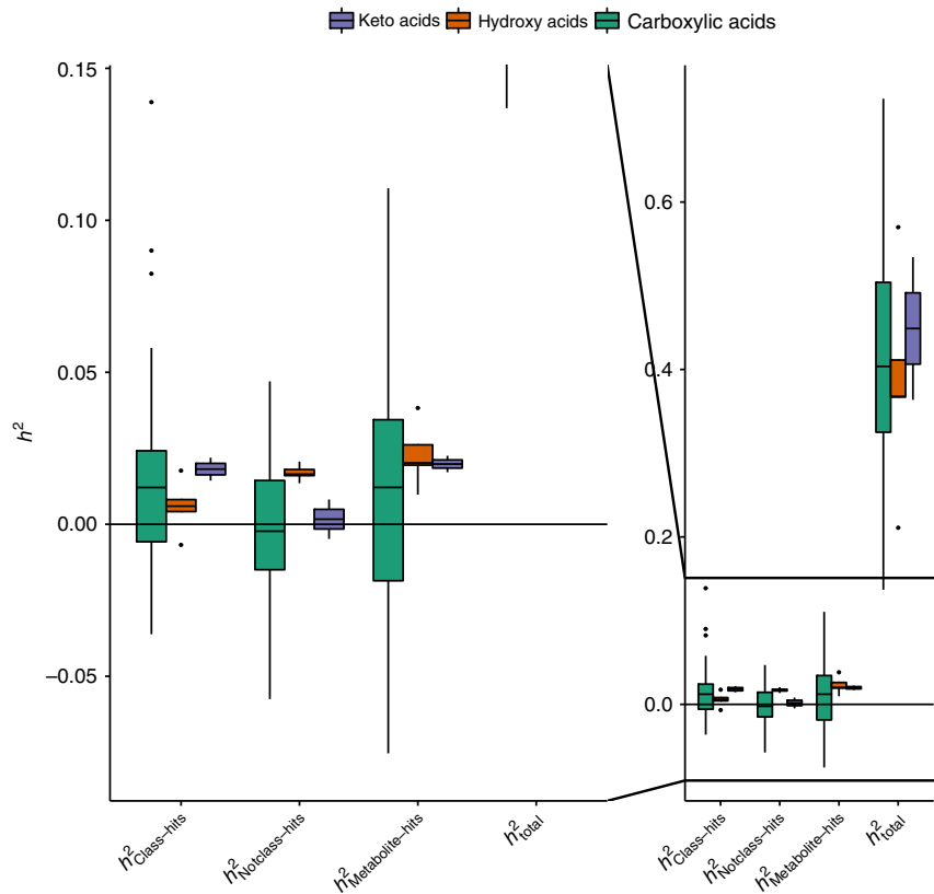
Fig. 2 Heritability of all 52 carboxylic acids by class. Box- and dotplots of the h^2_{\text{total}} and h^2_{\text{Metabolite-hits}} for all 52 successfully analyzed carboxylic acids and derivatives across all metabolomics platforms by class. The left-hand side of the figure is a close-up of the -0.08 to 0.15 part of the heritability range, focusing on the h^2_{\text{Class-hits}} and h^2_{\text{Notclass-hits}} estimates. The boxes denote the 25th and 75th percentile (bottom and top of box), and median value (horizontal band inside box). The whiskers indicate the values observed within up to 1.5 times the interquartile range above and below the box. The purple, orange and green boxes denote the keto acid, hydroxyl acid and carboxylic acid classes, respectively. Supplementary Data 3 provides the estimates for each of the individual metabolites.
