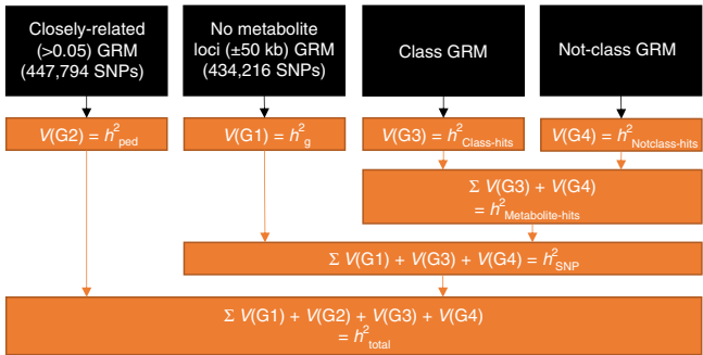
Fig. 1 Overview of the four-variance component models. Overview of the SNP-filtering and GRM construction can be found in Supplementary Fig. 1 and is explained in details in the Methods. This figure describes which GRMs (black boxes) are used to calculate which variance components (orange boxes) by drawing black arrows from the GRMs to the variance components. The variance components give rise to the four different heritability estimates: h^2_{\text{ped}} , h^2_{\text{g}} , h^2_{\text{Class-hits}} , and h^2_{\text{Notclass-hits}} (see Methods). The orange arrows indicate how the various variance components are summed to obtain estimates for h^2_{\text{Metabolite-hits}} , h^2_{\text{SNP}} , and h^2_{\text{total}} (see Methods).
