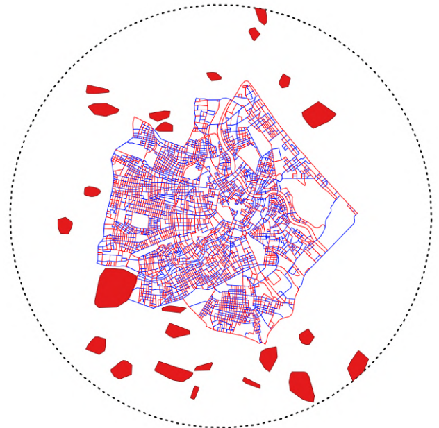
Fig. 5: Overview of the constrained airspace structure used within the decentralised concept, with red and blue streets having different cruise layer height allocations.
