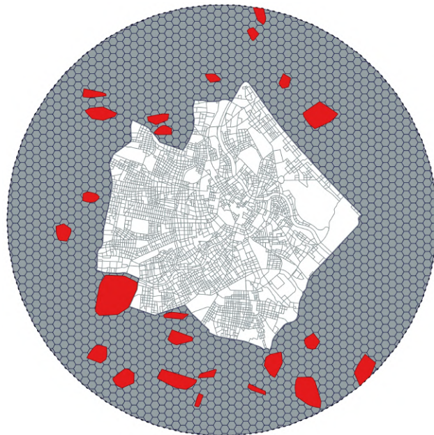
Fig. 1: Centralised concept airspace structure, with hexagonal cells in open airspace. The red polygons are geofences areas of open airspace.
