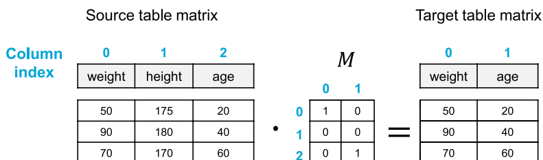
Fig. 2 An example of projection as matrix multiplication
