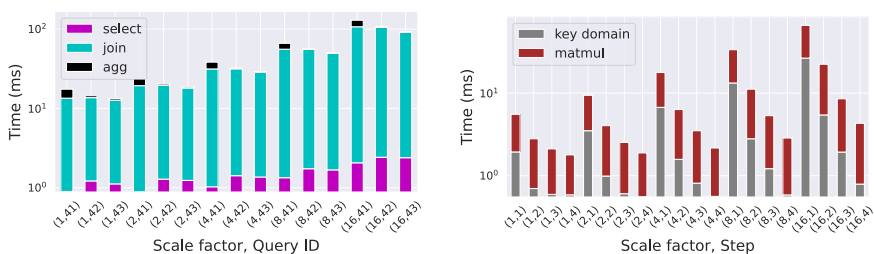
(a) Performance breakdown for queries w.r.t different scale factors. We take query group 4 as an example.
