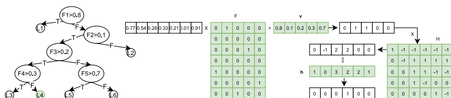
Fig. 4 Prediction with a decision tree with linear algebraic representation adapted from [19]
