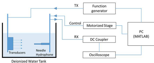
Fig. 4. Diagram of the measurement setup
