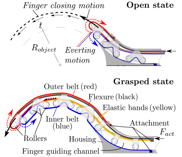
Fig. 2. Cross-sectional view of a DBCF-EM finger in the open and grasped states. Two everting belts (red, blue), guided by rollers, follow the curved flexure (black) and are fixed to the housing and flexure base via an elastic band (yellow). During grasp setting, the flexure is pushed outward the housing channel, restoring its curvature and following a circular path while driving the belts eversion motion from the tip along its outer sides to reduce shear with the environment.
